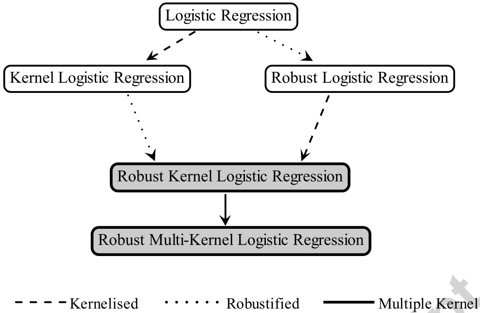
Fig. 1. Genealogy of the robust Kernel Logistic Regression and the robust Multi-Kernel Logistic Regression methods. The highlighted boxes are the classifiers proposed in this paper. Note that there are two paths to arrive at the robust Kernel Logistic Regression.
