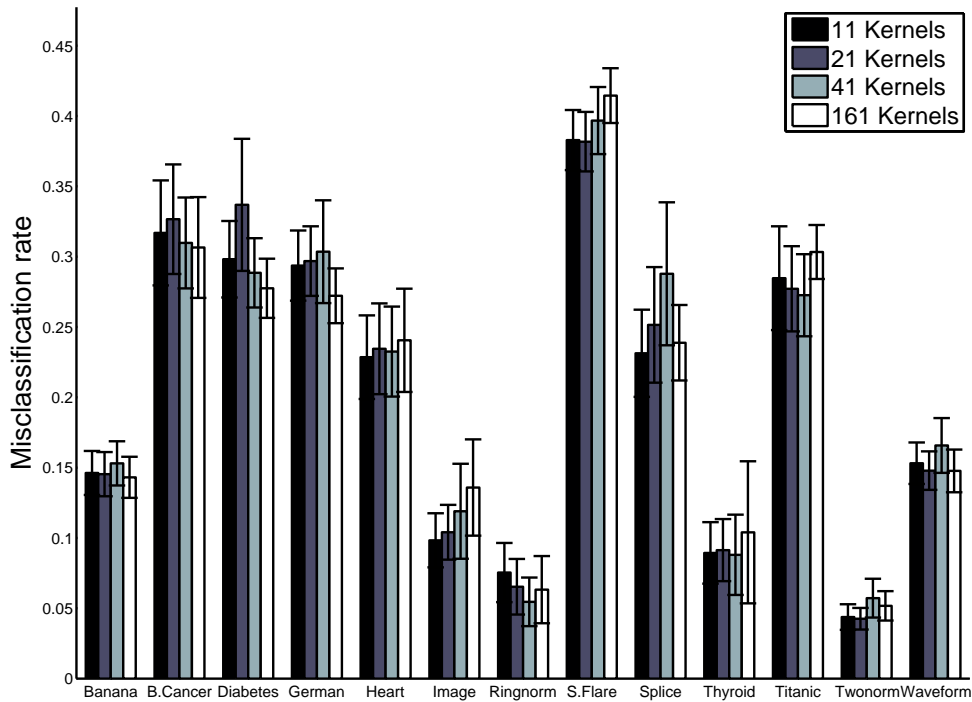
Fig. 5. Comparison of the different kernel set size at 30% level, averaged over 20 random runs.
