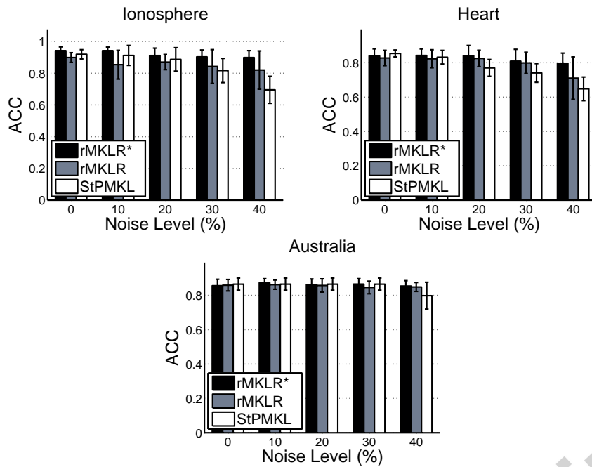
Fig. 6. Comparison of classification accuracy (ACC) with noise level ranging from 0% to 40%.
