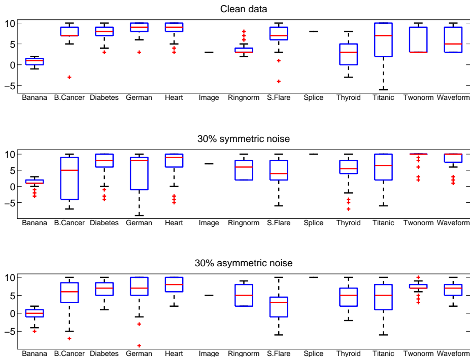
Fig. 4. Comparison of the medians of the kernel widths selected using clean data and two types of label noise at 30% level, averaged over 10 independent runs. Cross-validation was done using noisy validation set
