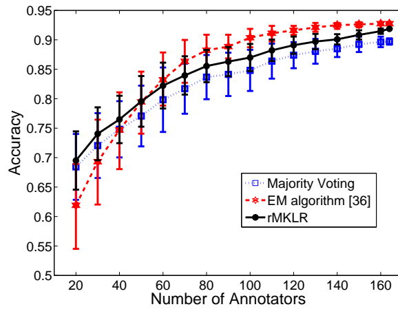
Fig. 7. Accuracy vs number of annotators in Textual Entailment recognition task. Each result is obtained by 100 independent draws without replacement from the total of 164 annotators.
