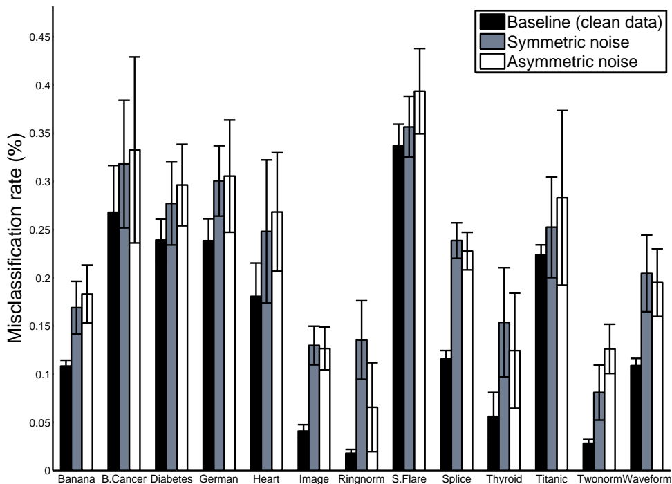
Fig. 2. Effect of 30% symmetric and asymmetric noise to traditional KLR, compared against clean baseline.
