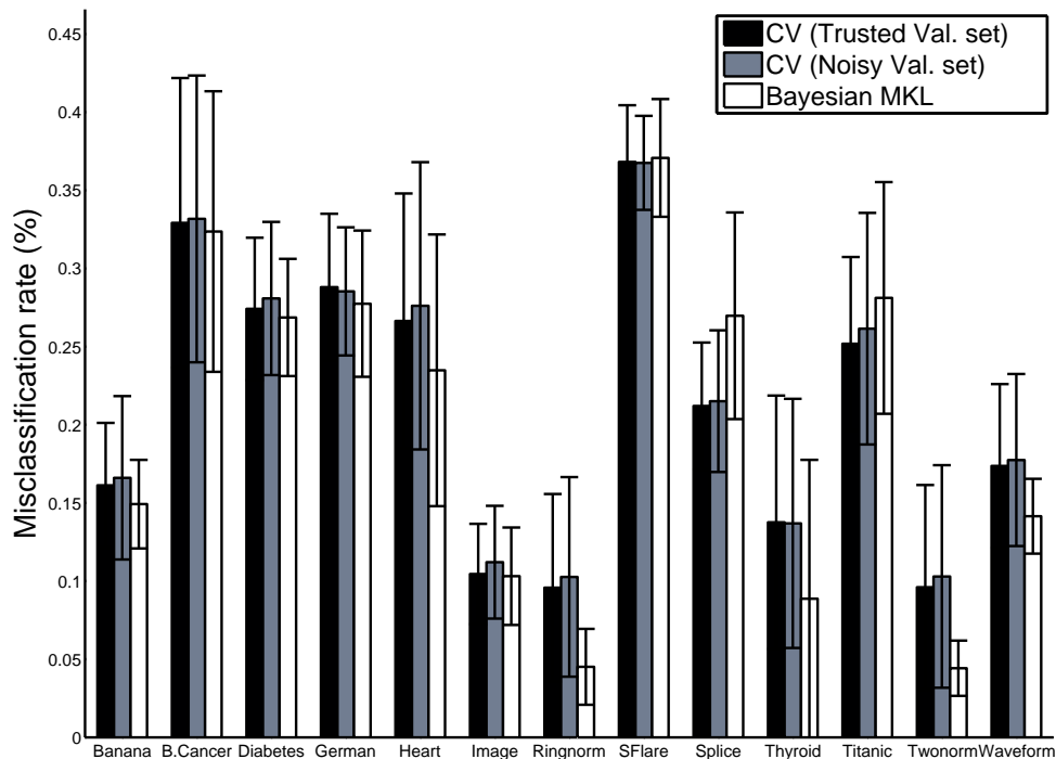
Fig. 3. Cross-validation for kernel width selection on different validation sets versus MKL with Bayesian regularisation.
