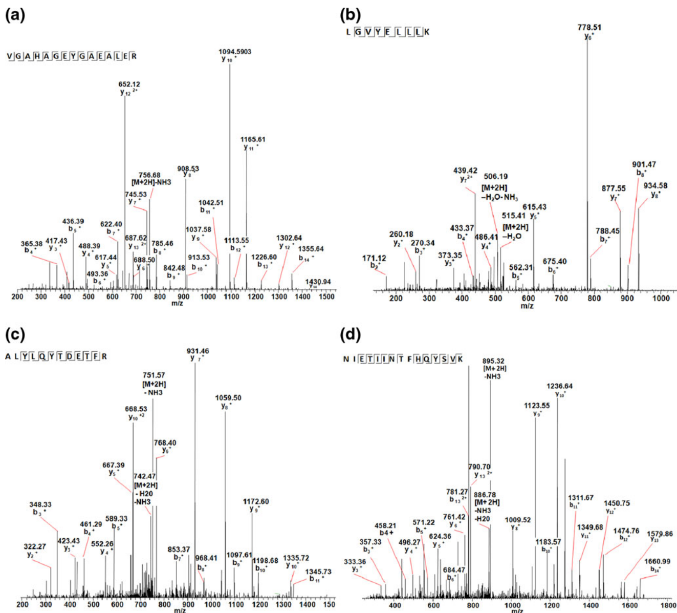
Figure 3. (a) CID MS/MS spectrum of peptide VG[A]H[A]G[E]Y[G]A[E]A[L]E[R] in the +2 charge state, from alpha chain of hemoglobin, a very high abundance protein. (b) CID MS/MS spectrum of peptide L[G]V[Y]E[L]L[L]K in the +2 charge state, from inter alpha trypsin inhibitor H4, a medium abundance protein. (c) CID MS/MS spectrum of peptide A[L]Y[L]Q[Y]T[D]E[T]F[R] in the +2 charge state from ceruloplasmin, a medium abundance protein and biomarker of Wilson's disease. (d) CID MS/MS spectrum of peptide N[I]E[T]I[N]T[F]H[Q]Y[S]V[K] in the +2 charge state from protein S100 A9, a very low abundance protein
