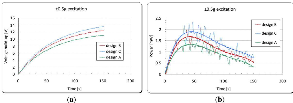
Figure 21. (a) Voltage build-up in a 2,200 \mu F capacitor and (b) the corresponding generated power by the energy harvester under \pm 0.5 g acceleration of excitation.
