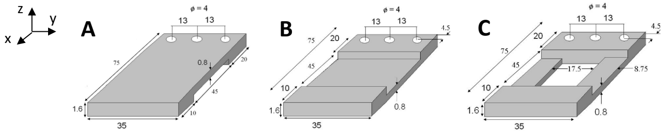
Figure 8. Configuration of the three cantilevers (all dimensions are in mm).
