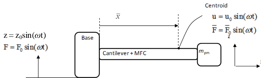
Figure 11. Harmonic excitation of the vibration-based energy harvester.
