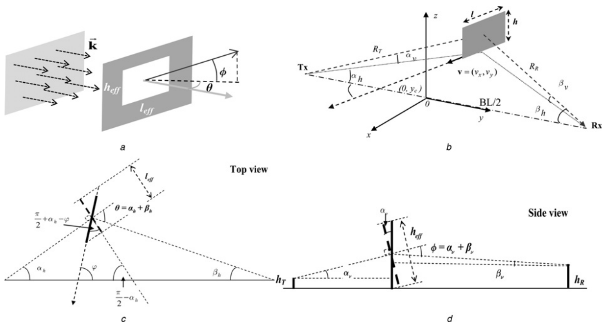
Fig. 2 Geometries for the calculation of the FS CS of moving target with rectangular cross-section
