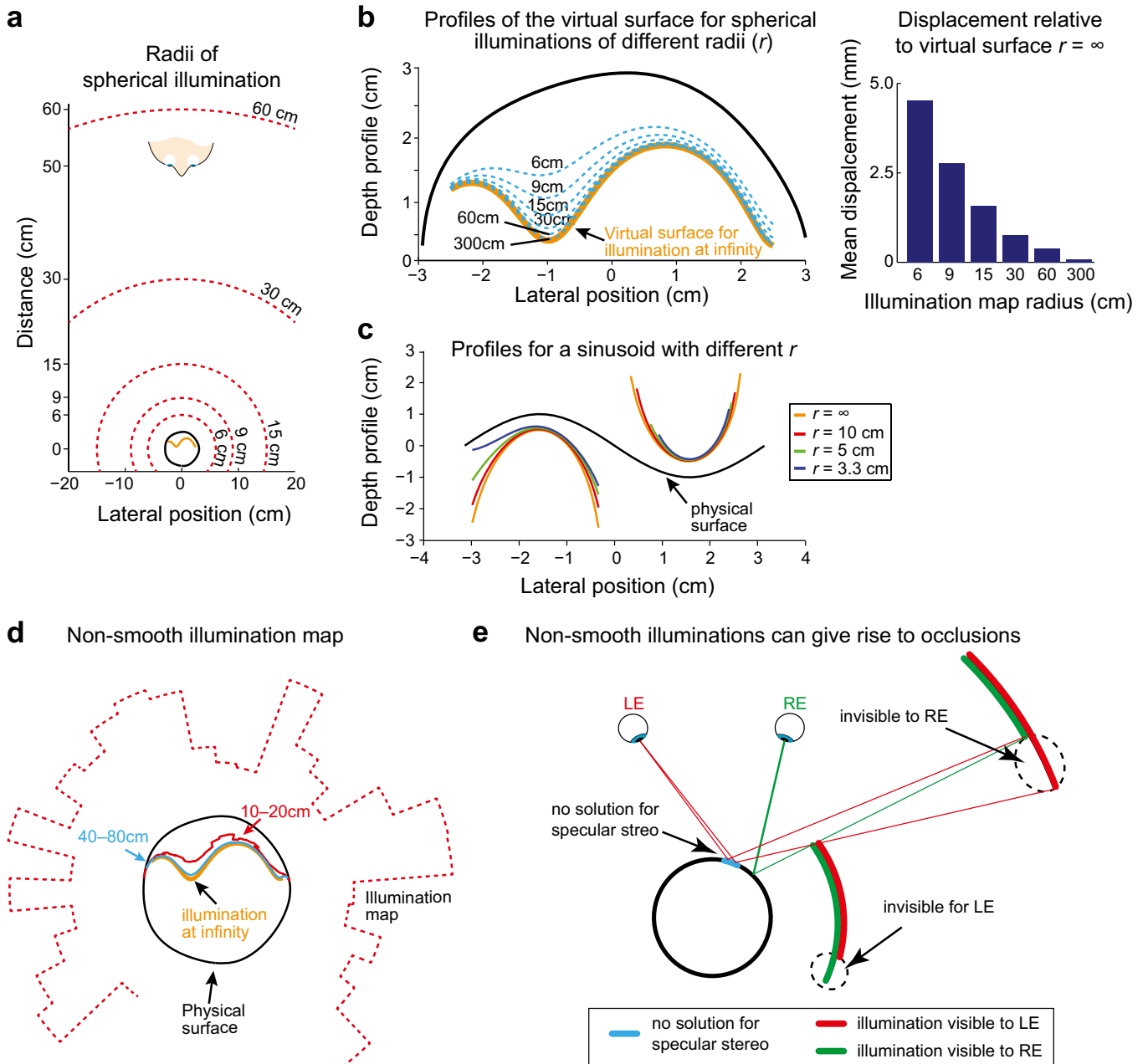
Fig. 55. Effect of illumination distance on the location of the virtual surface. (A) Schematic of the viewing geometry and illumination distances. (B) Virtual surfaces produced by illumination spheres of different radii. Solid orange line shows the profile obtained for illumination at infinity. Virtual surface changes systematically as the illumination gets closer to the object (dotted blue lines). We quantify the difference between the mean depth of the virtual surface at infinity and the other illumination distances (bar graph on Right ). (C) Virtual surfaces for a sinusoidal surface that contains both convexities and concavities. (D) Virtual surface under conditions of nonsmooth illumination for a nearby (10–20 cm) and intermediate (40–80 cm) illumination map. (E) Illustration of the potential for occlusion and nonmatchable features arising from specular reflection.
