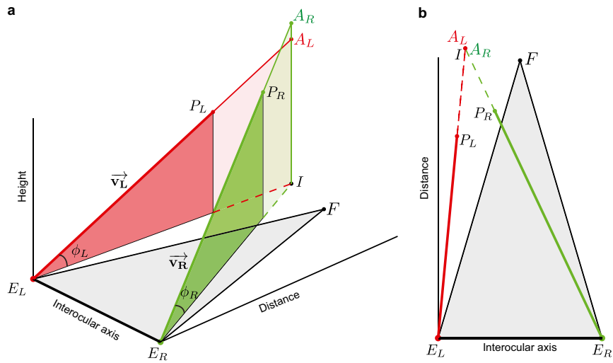
Fig. S1. Estimating depths for nonintersecting view vectors. (A) Three-dimensional view. The viewer fixates point F . P_L and P_R represent the two surface locations that reflect a given point in the environment ( P ) into the left and right eyes. The view vectors passing through these two points ( \vec{v}_L and \vec{v}_R ) do not intersect in 3D. We can define a virtual point for the left and right eyes ( A_R and A_L ) based on establishing a match using a projection into the fixation plane. We define virtual point ( A ) as the average of these two positions in 3D space. (B) Plan view. Assuming the visual system uses only the horizontal component of the disparity is equivalent to projecting the view vectors into the fixation plane, where they now intersect at point I . The virtual points ( A_L and A_R ) are defined as the projection of I back onto the 3D view vectors for the left and right eyes, respectively.
