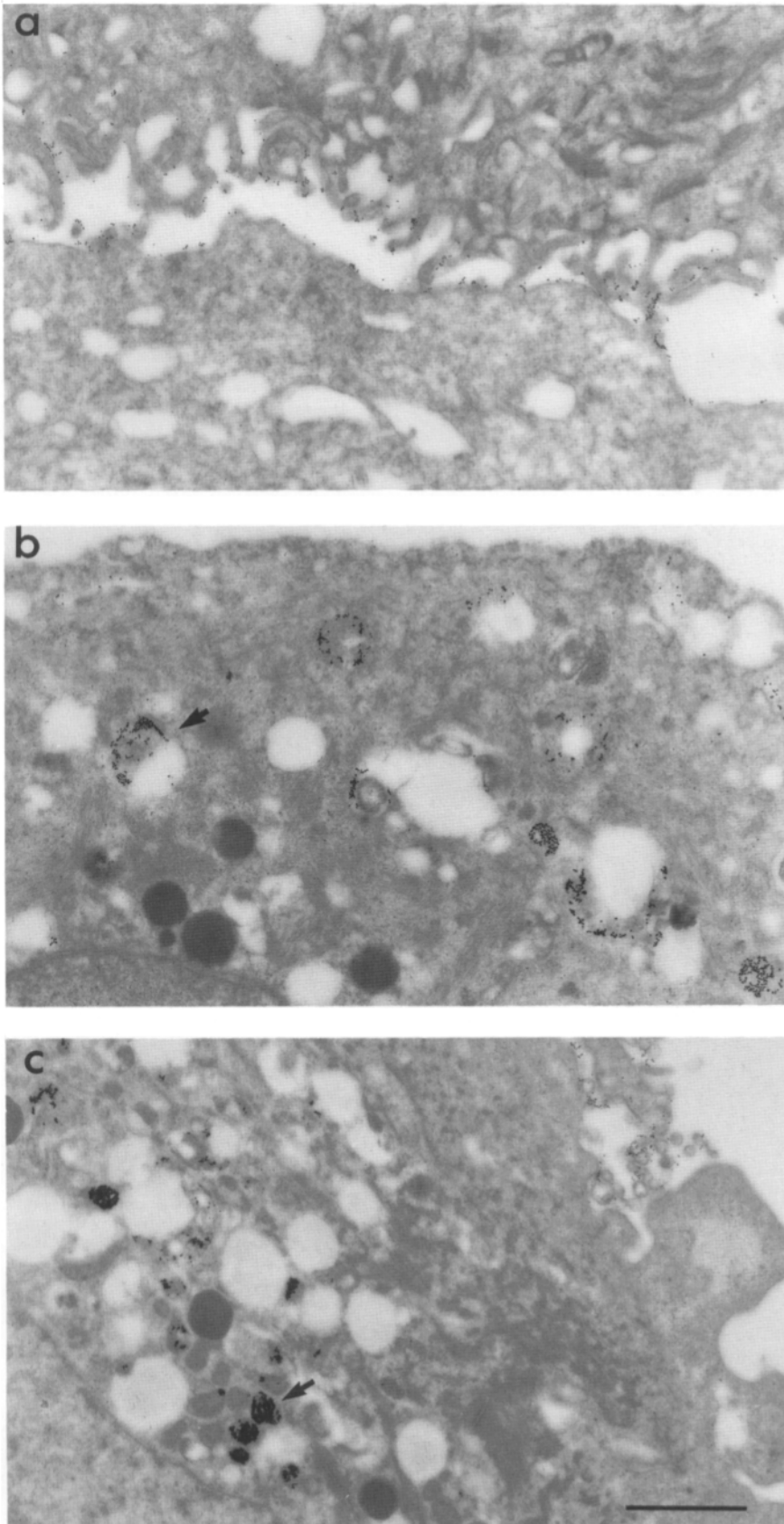
Figure 5. Immunogold labeling of keratinocytes with antibody to \alpha_3\beta_1 . (a) Freshly harvested cells. (b and c) After 22 h in suspension. Arrows indicate endosome (b) and lysosome (c). Bar, 1 \mu\text{m} in a, 0.7 \mu\text{m} in b, and 0.8 \mu\text{m} in c.
