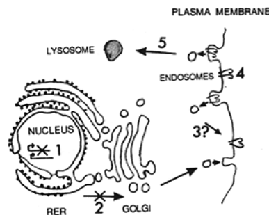
Figure 7. Model of the different levels of regulation of \beta_1 integrins in keratinocytes undergoing terminal differentiation, based on the present results and previously published data. (1) Inhibition of transcription (Hotchin and Watt, 1992). (2) Inhibition of intracellular transport. (3) Recycling of active receptor? (4) Inactivation of receptor, probably resulting from a change in receptor conformation (Hotchin et al., 1993). (5) Endocytosis of inactive receptor and degradation in lysosomes. \alpha , active form of \beta_1 integrin; \beta , inactive form of \beta_1 integrin. Structure of cell redrawn from Alberts et al. (1989).
