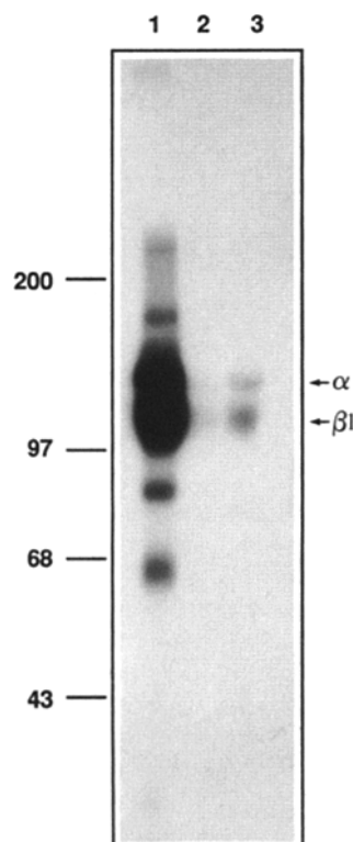
Figure 4. Internalization of cell surface integrins. Freshly harvested keratinocytes were labeled with [ ^{125} I]iodine and either extracted and immunoprecipitated with anti- \beta_1 immediately (lane 1) or placed in suspension (lanes 2 and 3). After 24 h in suspension, cells were incubated with anti- \beta_1 and extracted. Anti- \beta_1 with bound integrin was collected for immunoprecipitation to detect surface integrins (lane 2), and the lysate was reimmunoprecipitated with anti- \beta_1 to detect internalized integrin (lane 3). Positions of molecular mass standards and integrin subunits are indicated. Gel was run nonreduced.
