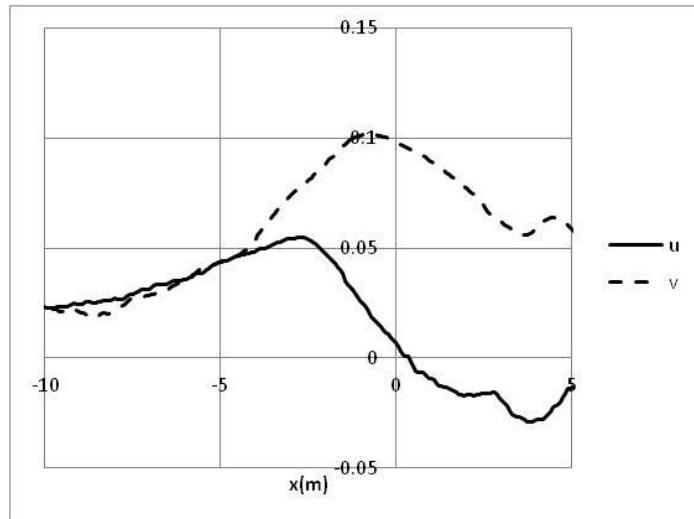
Figure 22. Slipstream velocity traces around the nose of an ICE-1 train, 2.85m from the track centre line, 0.5m above top of rail [11] - the graph shows the longitudinal (u) and lateral (v) components of horizontal slipstream velocity normalised by the train speed; distance is measured from an arbitrary point close to the train nose
