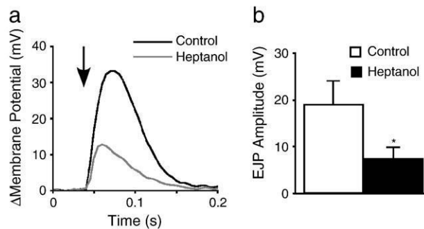
Fig. 4. The effect of heptanol on EJPs in guinea pig vas deferens. There was a decrease in EJP amplitude on exposure to heptanol (2 mM) in mice. (a) shows representative EJPs before and after heptanol exposure. (b) shows that the mean EJP amplitude decreased in the presence of heptanol ( n=6 ). A single field stimulus was applied at the arrow. * denotes P<0.05 compared with control.
