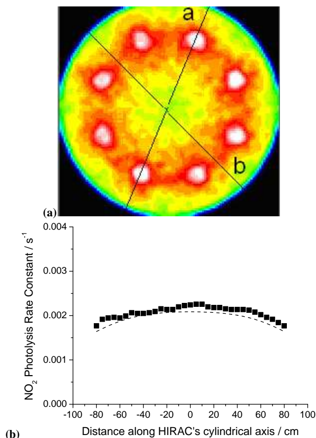
Fig. 4. (a) Pictorial results of a typical ray trace simulation, showing the relative energy incident on a plane that bisects HIRAC, and is parallel to its end flanges. The lines a and b in the figure correspond to the results plotted in Figs. 3a and b. (b) Comparison of the analytical form derived to describe \text{NO}_2 photolysis as a function of position along HIRAC's cylindrical symmetry axis (—), and the multireflection ray trace results (■) carried out on the HIRAC solid model.
