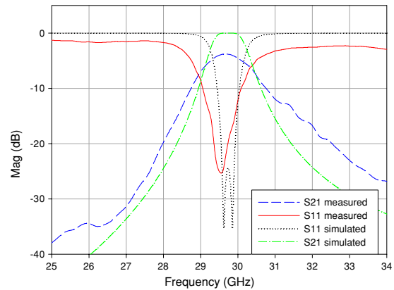
Figure 3. Response of the prototype filter.
