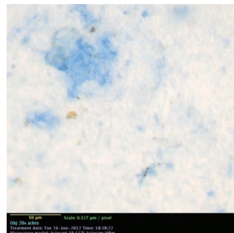
▲ Figure 3: CSP particles from SML of the fjord
