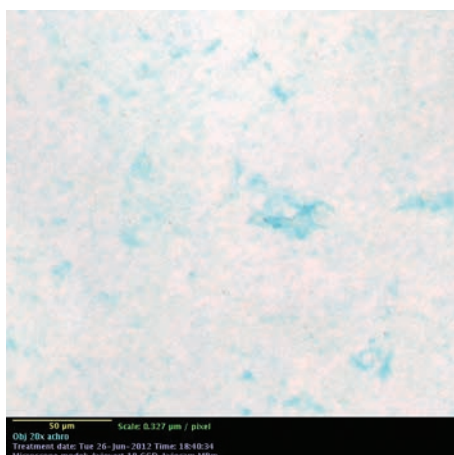
▲ Figure 2: TEP particles from SML of the fjord
