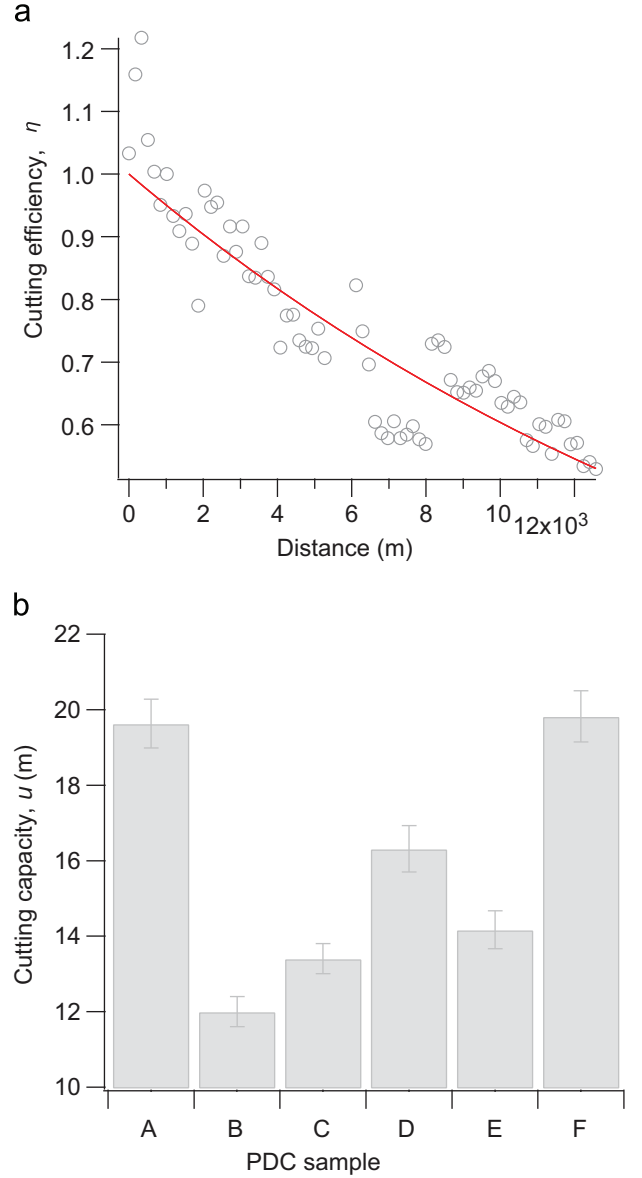
Fig. 6. Cutting efficiency analysis: (a) Cutting efficiency vs. distance model for sample F; (b) cutting capacity results.
