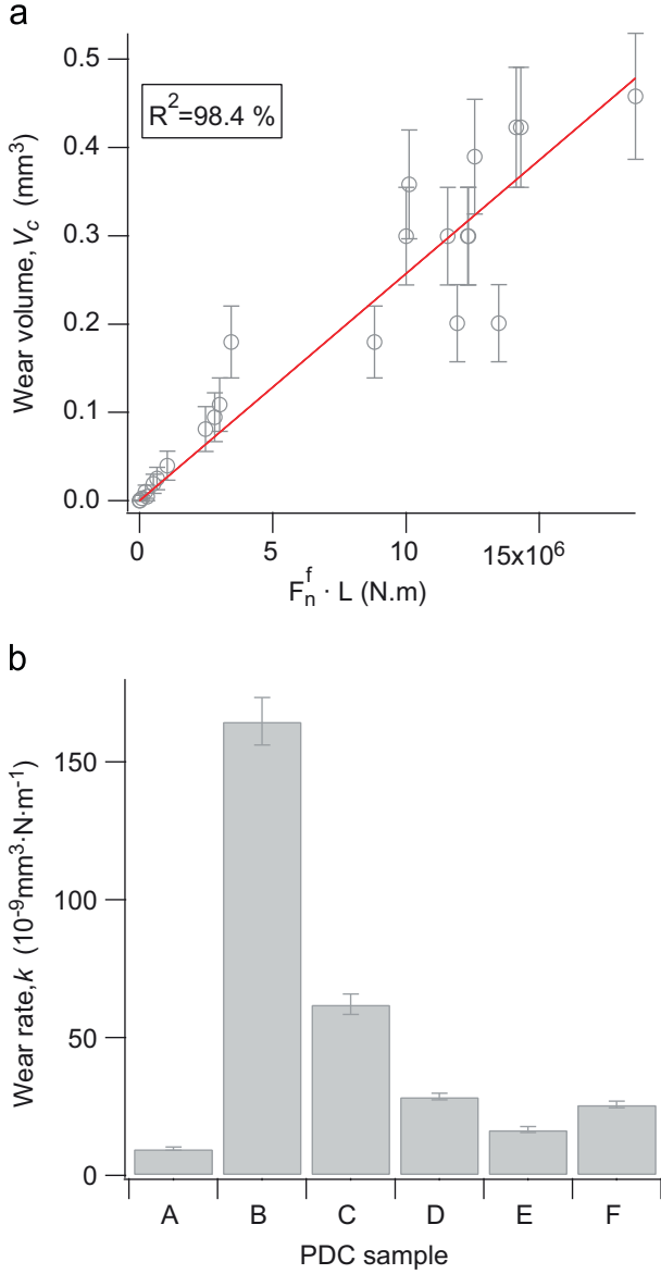
Fig. 5. Wear rate evaluation: (a) Archard's model applied to sample F; (b) wear rates results.
