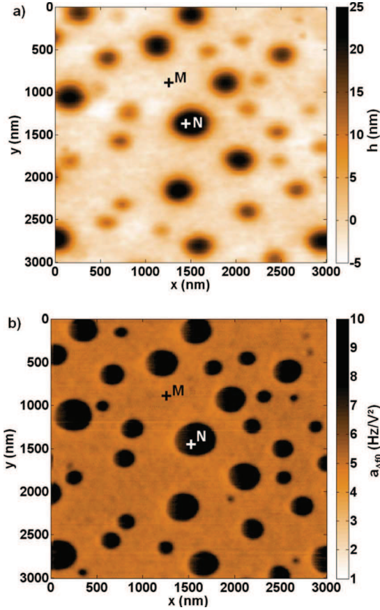
FIG. 3. (Color online) (a) Topography of the PVAc/PS film. (b) Corresponding map of the coefficient a_{\Delta f_0} . Values of t and a_{\Delta f_0} at points M (PS matrix) and N (PVAc nodule) have been reported in Fig. 1 where they have been interpolated with ECM simulated curves in order to extract the corresponding value of \epsilon_r .
