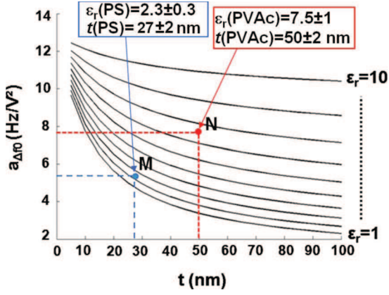
FIG. 1. (Color online) Numerical simulations based on ECM of the curves a_{\Delta f_0}(t, \epsilon_r) , where t is the sample thickness and \epsilon_r is the relative dielectric permittivity, for a tip radius R=19 nm and a tip-sample distance z_0=18 nm. M(t, a_{\Delta f_0}) and N(t, a_{\Delta f_0}) are typical points obtained from AFM topography and EFM images (Fig. 3), respectively, on the PS matrix and the PVAc nodules of the studied polymer blend thin film. \epsilon_r can be deduced by interpolating these points with simulated curves.
