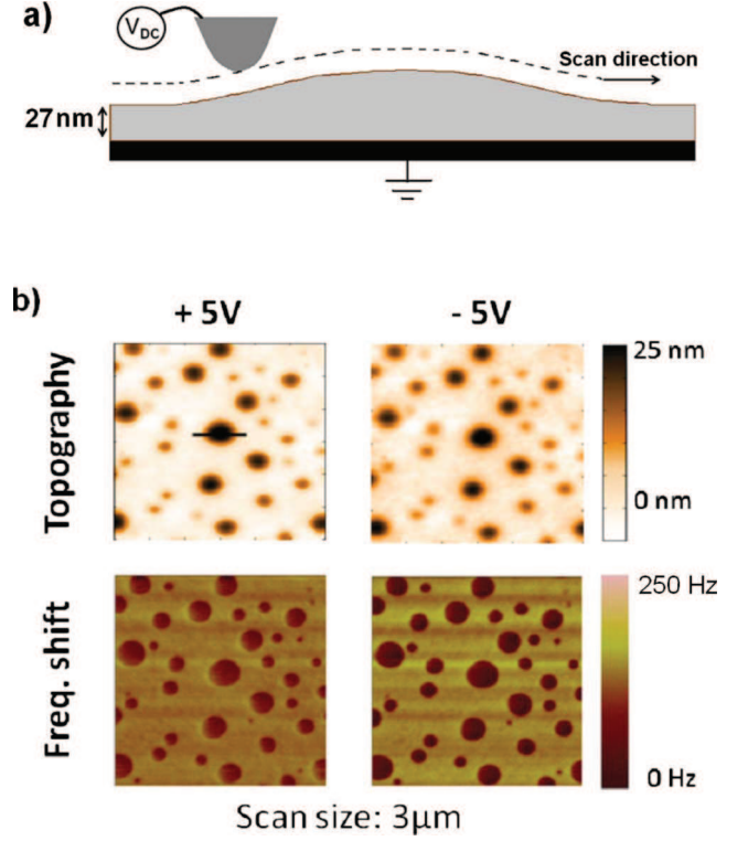
FIG. 2. (Color online) (a) Typical topographic profile of PVAc islands in a PS matrix. Both tip and polymer film are represented at the same scale. The dash line represents the tip motion during the second scan. (b) Topography and frequency shift measured by the double pass method at +5 and -5 V on the PVAc/PS films. The black line corresponds to the profile appearing in (a).
