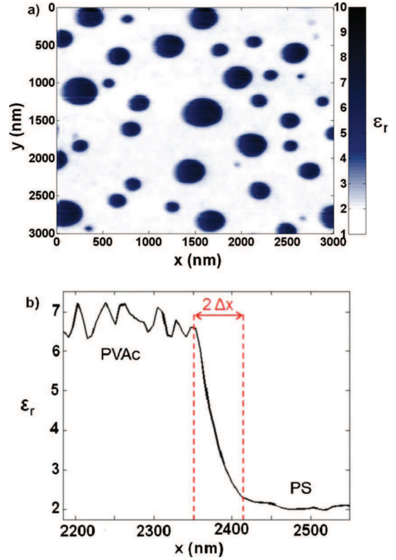
FIG. 4. (Color online) (a) Map of the dielectric constant of the PVAc/PS film obtained by processing images shown in Fig. 3. (b) Typical profile of the dielectric permittivity across the PVAc/PS interface.
