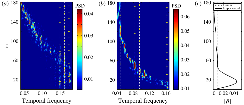
FIGURE 4. (Colour online) (a,b) PSD of the cross-flow component of flow velocity along a spanwise line in the wake, in the (a) narrowband (linear shear flow, (x, y) = (20, 0) ) and (b) broadband (exponential shear flow, (x, y) = (15, 0) ) response cases. Dashed lines indicate the frequencies of the cross-flow vibrations identified in figure 2 and yellow crosses show the local minima of the cross-flow vibration PSD, at each frequency. (c) Spanwise evolution of the magnitude of the inflow velocity profile shear rate.
