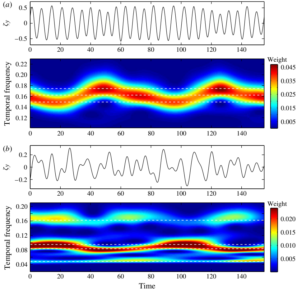
FIGURE 3. Selected time series of the cross-flow displacement and corresponding frequency content as a function of time (scalogram), in the (a) narrowband (linear shear flow, z = 7.5 ) and (b) broadband (exponential shear flow, z = 9.4 ) response cases. Dashed lines denote the vibration frequencies identified in figure 2.
