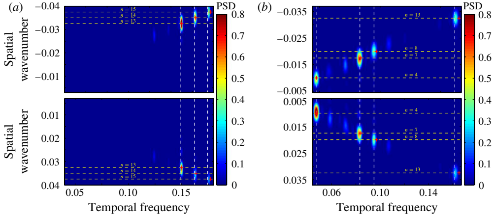
FIGURE 2. Spatiotemporal spectral analysis of the cross-flow displacement in the (a) linear and (b) exponential shear flow cases. Selected vibration frequencies are identified by white vertical dashed lines. The wavenumbers of selected sine Fourier modes are indicated by yellow horizontal dashed lines. Red crosses denote the natural frequencies associated with these wavenumbers.
