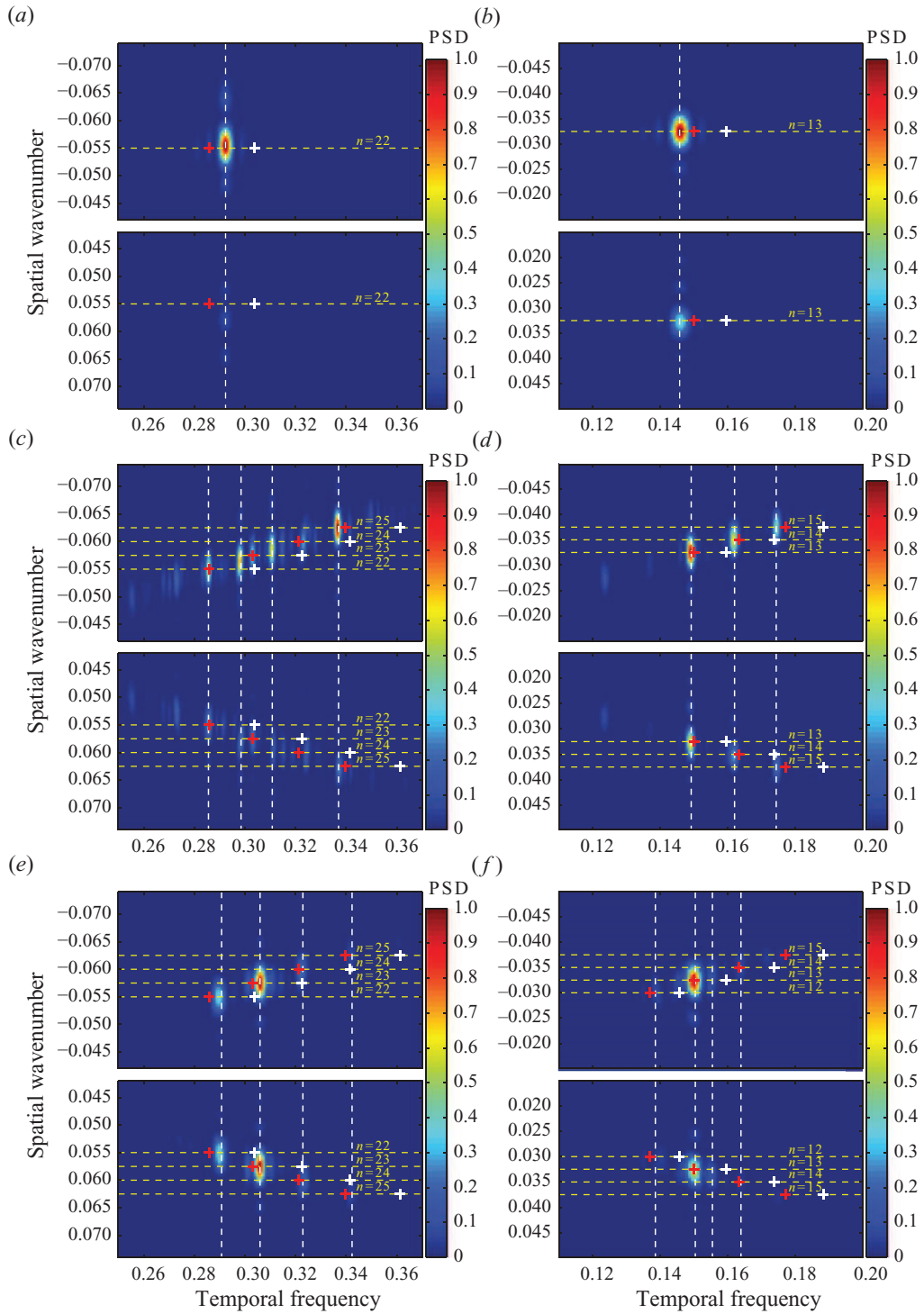
FIGURE 7. Spatio-temporal spectral analysis of (a,c,e) in-line displacement fluctuation and (b,d,f) cross-flow displacement at (a,b) Re_m = 110 , (c,d) Re_m = 330 and (e,f) Re_m = 1100 . The white vertical dashed lines denote the frequencies identified in figures 5 and 6. The wavenumbers of selected sine Fourier modes are indicated by yellow horizontal dashed lines. The white (red) crosses denote the natural (modified) frequencies associated with these wavenumbers.
