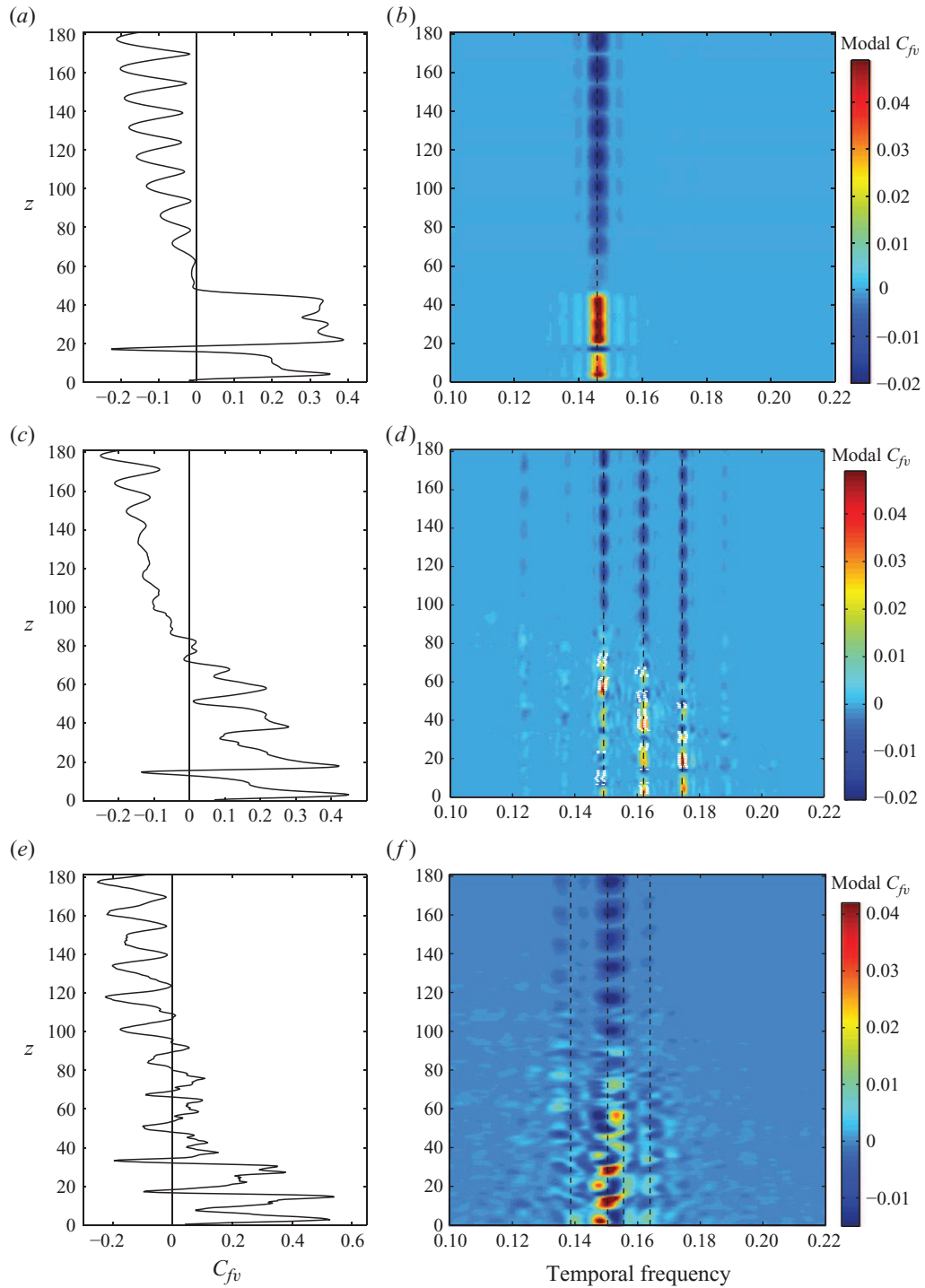
FIGURE 22. Force coefficient in phase with the cylinder velocity along the cylinder span: (a,c,e) total and (b,d,f) frequency decomposition, at (a,b) Re_m = 110 , (c,d) Re_m = 330 and (e,f) Re_m = 1100 . The black dashed lines indicate the frequencies identified in figure 6. In (d), the white dashes indicate the local predominant vortex shedding frequency obtained from figure 13 (d).
