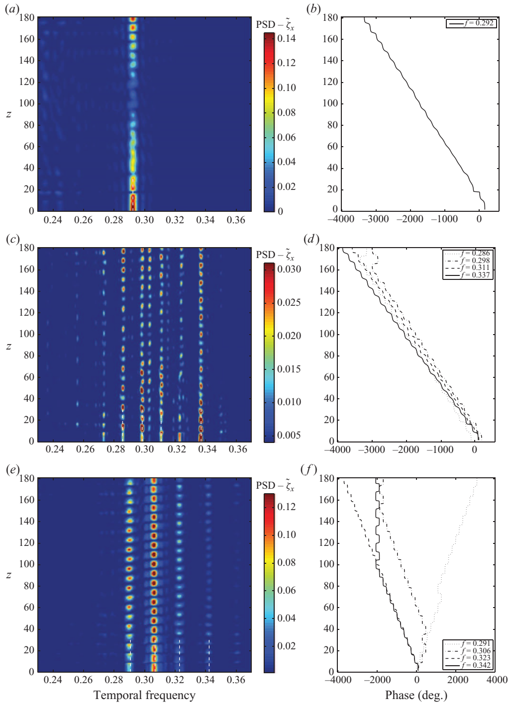
FIGURE 5. Temporal spectral analysis of in-line displacement fluctuation: (a, c, e) PSD of \tilde{\zeta}_x along the cylinder span and (b, d, f) spanwise evolution of selected temporal mode phase angles at (a, b) Re_m = 110 , (c, d) Re_m = 330 and (e, f) Re_m = 1100 .
