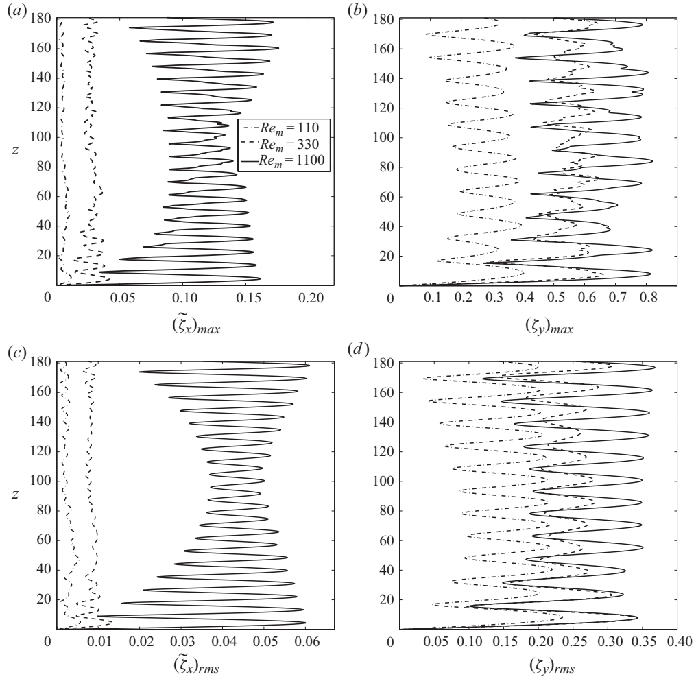
FIGURE 4. (a,b) Maximum and (c,d) r.m.s. values of (a,c) in-line displacement fluctuation and (b,d) cross-flow displacement along the cylinder span.
