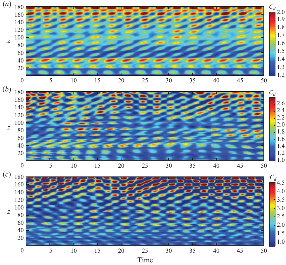
FIGURE 19. Temporal evolution of drag coefficient along the cylinder span at (a) Re_m = 110 , (b) Re_m = 330 and (c) Re_m = 1100 .
