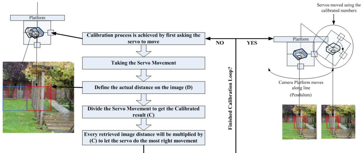
Figure 4.2 – Calibration loop
