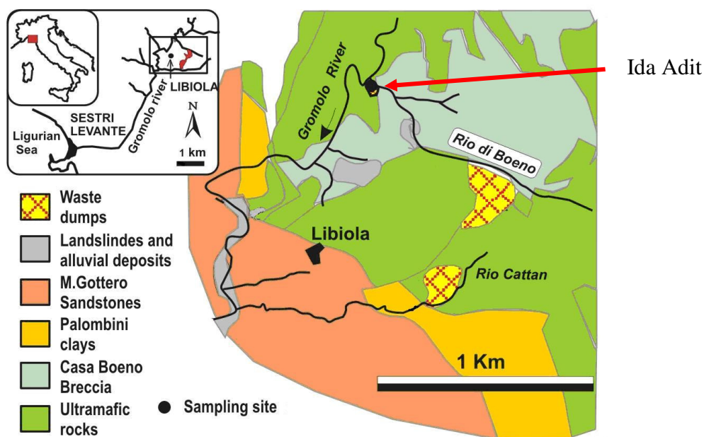
Figure 8.2. Geological map of the Libiola Fe-Cu mine, Italy. After: Dinelli et al. , 2007
