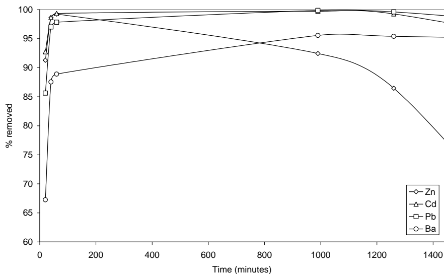
Figure 7.8. Removal of Zn, Cd, Ba and Pb from 1 L/minute Algavi (c) DS treatment plant at Bwlch during the first 1440 minutes (24 hours). Average inlet concentration: Zn ~25 mg/L, Cd ~64µg/L, Ba ~ 24 µg/L and Pb ~700 µg/L.
