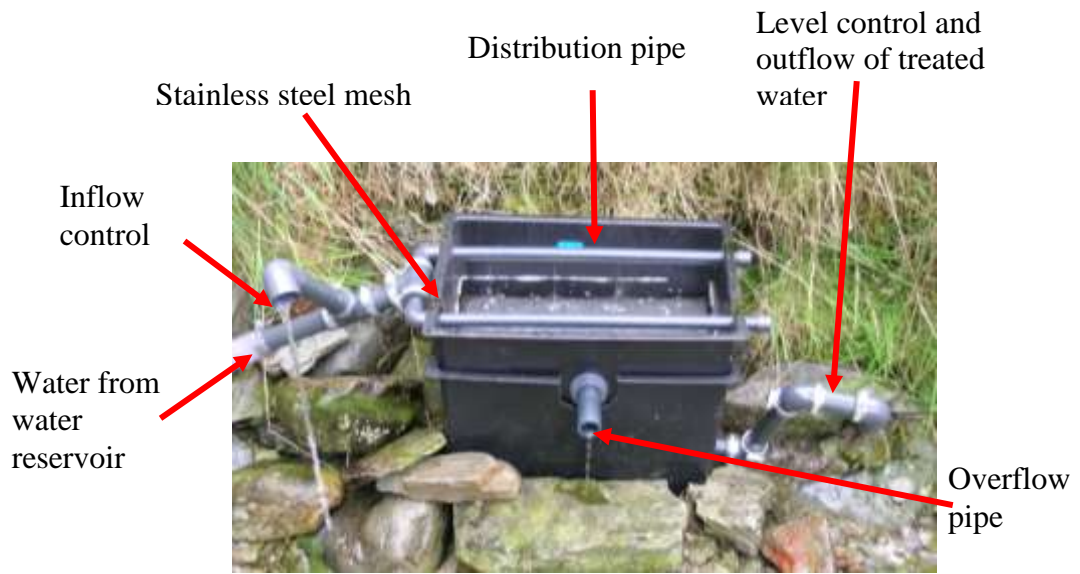
Figure 7.2. 1 L/minute treatment plant at Bwlch.
