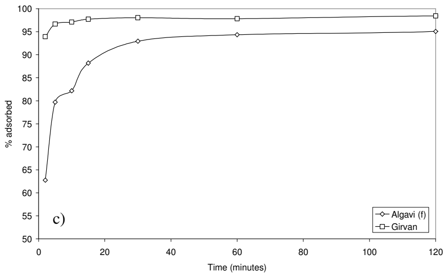
Figure 6.3. Adsorption of: a) Zn, b) Cd and c) Pb by 0.5 g Algavi (f) and Girvan (r) DS from Bwlch mine water over 120 minutes.
