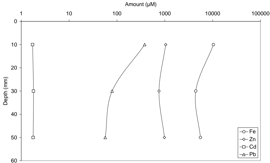
Figure 7.22. Amount of Fe, Zn, Cd and Pb ( \mu\text{M} ) within each 20 mm layer through the carbonate sand core from the Esgair Hir 1 L/minute treatment plant. The marker is placed in the centre of the layer i.e. the marker at 10 mm represents the amount of the layer 0-20 mm. Note the logarithmic scale.
