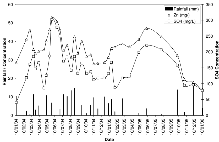
Figure 4.17. Zn and SO 4 concentrations at Bwlch.
