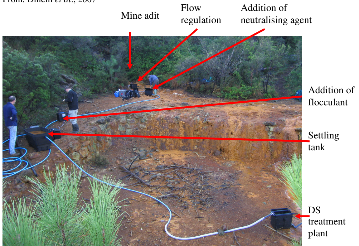
Figure 8.13. Photograph of the Ida adit pilot treatment plant system.
