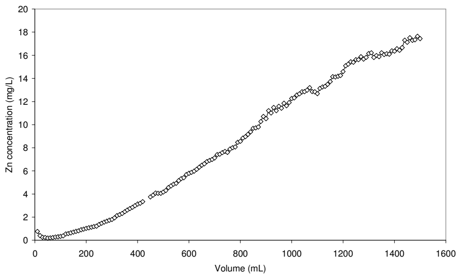
Figure 6.16. Concentration of Zn in the effluent after Bwlch mine water has flowed through a bed of 2.5 g Algavi (e) DS. Initial concentration of Zn is 36 mg/L.
