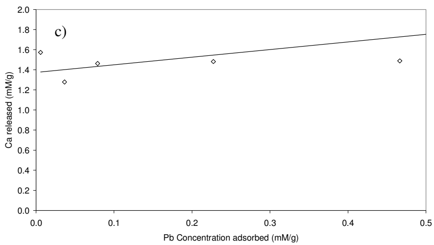
Figure 6.14. Relationship between: a) Zn, b) Cd and c) Pb adsorption and Ca release (mM/g) in single metal solutions by 0.5 g Algavi (f) DS.
