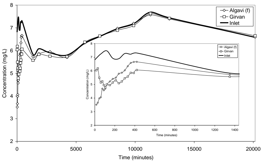
Figure 7.33. Concentration of Mg in the inlet and outlet waters of the Algavi (f) and Girvan DS 1 L/minute treatment plant at Bwlch. Inset: first 1440 minutes (24 hours).
