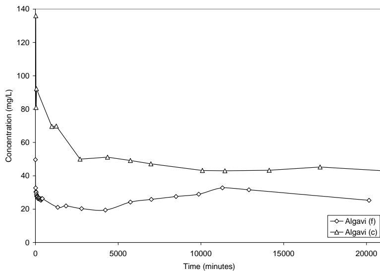
Figure 7.41. Ca in the outlet water of the \text{Algavi}_{(c)} and \text{Algavi}_{(f)} DS 1 L/minute treatment plant at Bwlch. Average inlet Ca concentrations: \text{Algavi}_{(c)} 40 mg/L; \text{Algavi}_{(f)} 26 mg/L.
