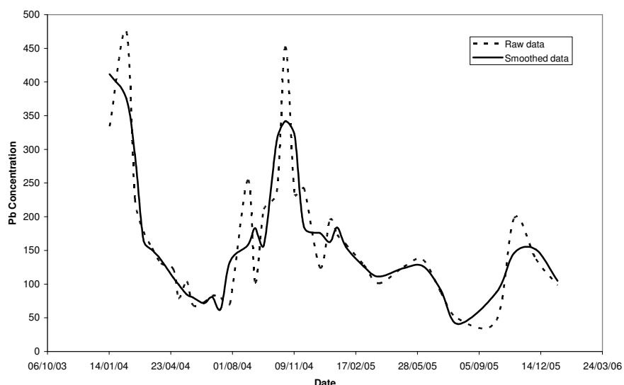
Figure 4.2. Comparison between raw and 5 term smoothed Pb concentrations at Alltycrib. Concentrations displayed in µg/L.
