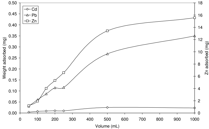
Figure 6.12. Weight of Zn, Cd and Pb adsorbed from Bwlch mine water by 0.5 g Algavi (f) DS. Initial concentration of Zn 27.9 mg/L, Cd 76.7 µg/L and Pb 667 µg/L.
