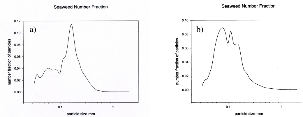
Figure 5.2. Grain size distribution: a) Girvan DS and b) Algavi DS.
