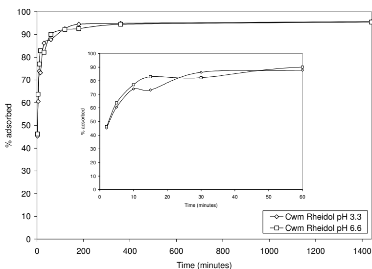
Figure 6.8. Adsorption of Zn from Cwm Rheidol mine waters at pH 3.3 and pH 6.6 over 1440 minutes. Inset: first 60 minutes. Initial concentrations of Zn: Cwm Rheidol pH 3.3 21.9 mg/L and Cwm Rheidol pH 6.6 21.5 mg/L.
