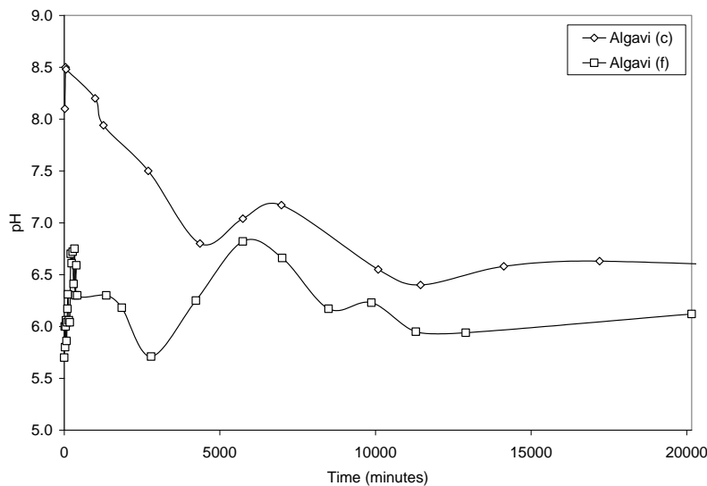
Figure 7.42. pH of the outlet water from the \text{Algavi}_{(c)} and \text{Algavi}_{(f)} DS treatment plant. Average inlet pH: \text{Algavi}_{(c)} 6.8; \text{Algavi}_{(f)} 6.2.
