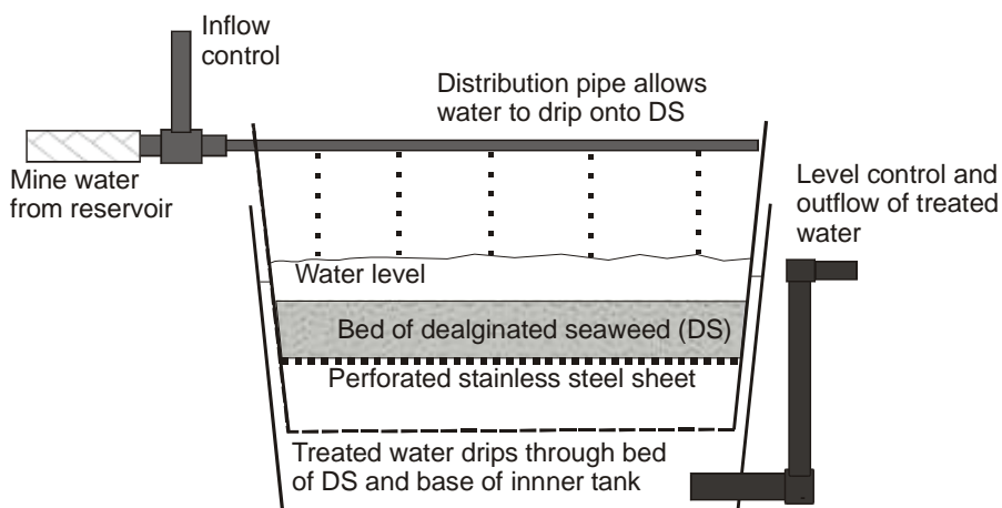
Figure 7.1. Schematic of the 1 L/minute treatment plant.
