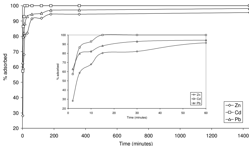
Figure 6.4. Adsorption of Zn, Cd and Pb from Bwlch mine water by Algavi (D) DS over 1440 minutes. Inset: first 60 minutes.
