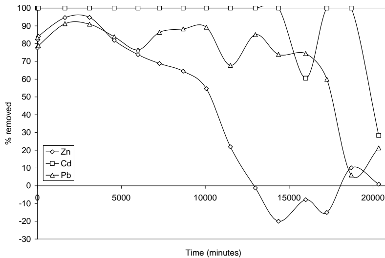
Figure 7.26. Removal of Zn, Cd and Pb from the 2 L/minute Algavi (t) (carbonate free) DS treatment plant at Alltycrib.
