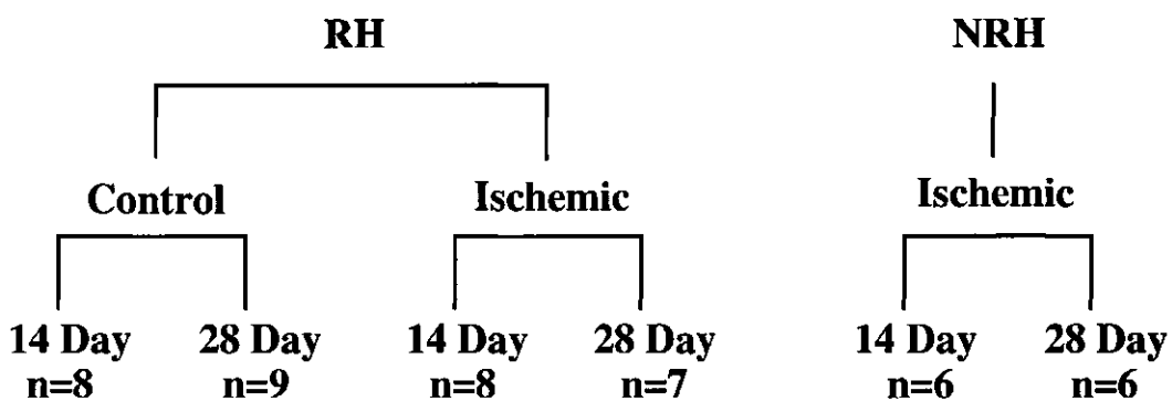
Figure 3.1: Experimental design for fourteen day (14-RH) delay Control and Ischemic Conditions, for twenty-eight day (28-RH) delay Control and Ischemic Conditions, and for Non-rehabilitation (NRH) Conditions.
