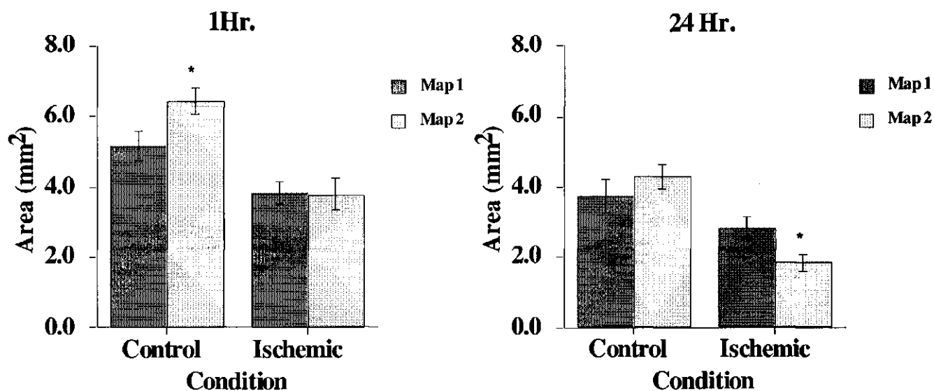
Figure 2.2 - Total area of CFA (mm 2 ) after 1 Hr (A) and 24 Hr (B). There is a significant increase in CFA area one hour following ICMS and a significant decrease in peri-infarct representation twenty-four hours following ischemia (*p<0.05; two-tailed, dependent Student's t-test).
