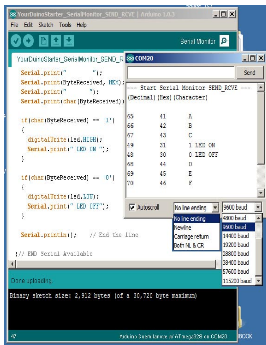
Figure 4.7: Serial Monitor of Arduino UNO
