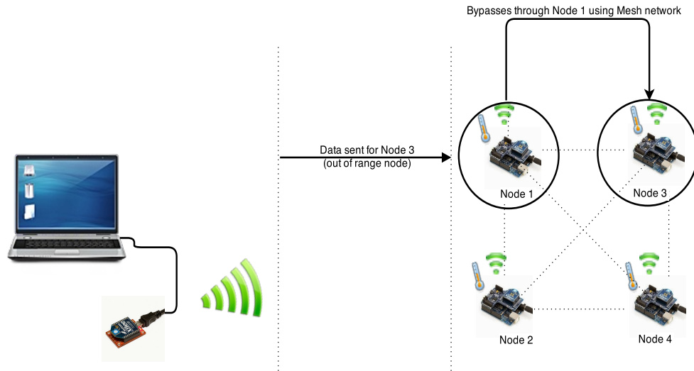
Figure 5.4: Using mesh network for performance analysis
