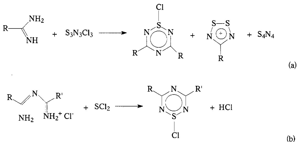
Figure 2.22 Synthetic routes to 1-chloro-1,2,4,6-thiatriazines
