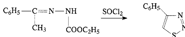
Figure 2.12 Synthetic route to 1,2,3-thiadiazoles
