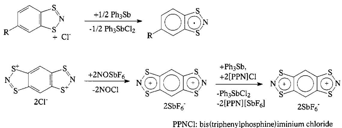
Figure 2.10 Synthetic routes to the 1,3,2-dithiazolyl radicals by reduction
