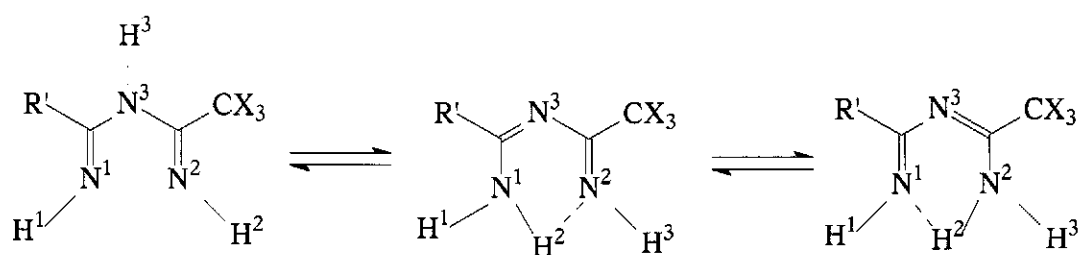
Figure 3.5 Tautomerism of N -imidoamidine
