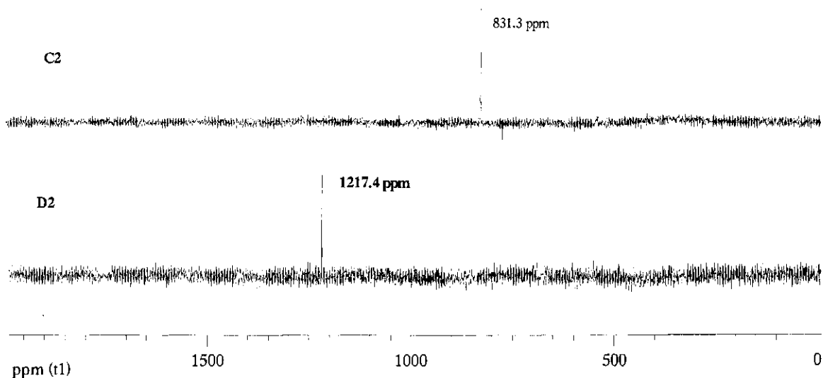
Figure 3.13 77 Se NMR of C2 (in DMSO) and D2 (in chloroform) using SeO 2 (in H 2 O) at +1306 ppm as external standard.
