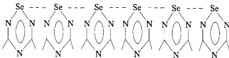
Figure 5.14 Packing arrangement for three selenotriazinyl dimers (a Ref3, b E10, c E9, d desired ordered packing arrangement)
