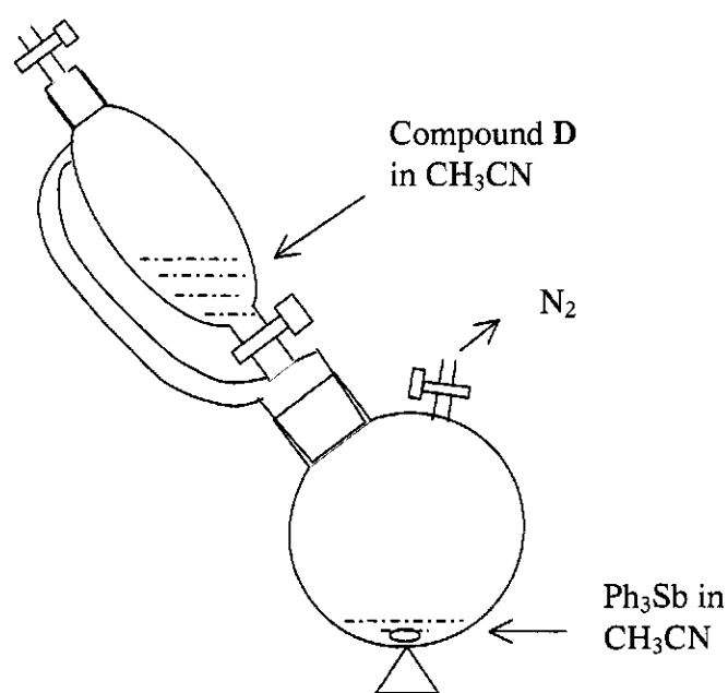
Figure 4.4 Apparatus to prepare and in-situ crystallize selenotriazinyl radicals
