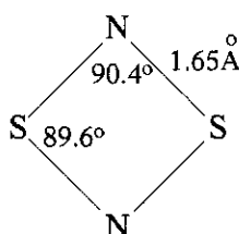
Figure 2.3 The structure of disulfur dinitride
