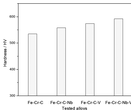
Figure 7: Hardness of the tested alloys Slika 7: Trdota preizkusnih zlitin
