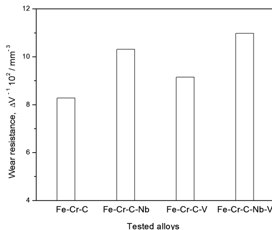
Figure 8: Wear resistance of the tested alloys Slika 8: Obrabna otpornost preizkusnih zlitin
