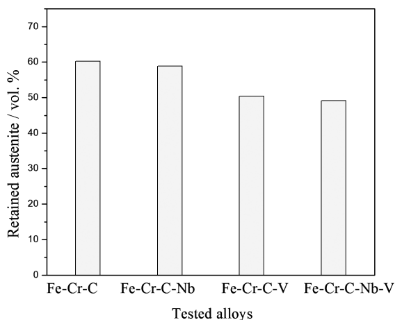
Figure 3: Volume fraction of the retained austenite in the tested alloys Slika 3: Volumenski delež zaostalega avstenita v preizkusnih zlitinah
