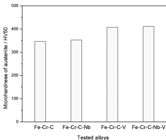
Figure 6: Microhardness of the tested alloys Slika 6: Mikrotvrdoća preizkusnih zlitin
