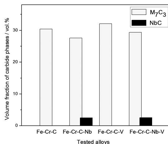
Figure 4: Volume fractions of carbide phases in the tested alloys Slika 4: Volumenski deleži karbidnih faz v preizkusnih zlitinah
