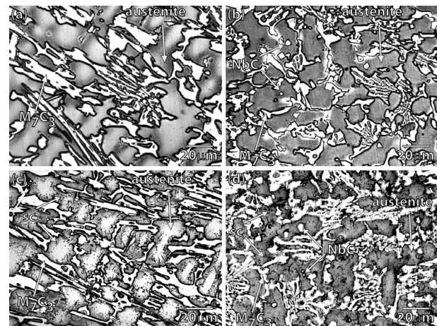
Figure 1: LM micrographs of the: a) basic Fe-Cr-C alloy, b) Fe-Cr-C-Nb alloy containing 1.58 % Nb, c) Fe-Cr-C-V alloy containing 1.55 % V and d) Fe-Cr-C-Nb-V alloy containing 1.53 % Nb and 1.47 % V
