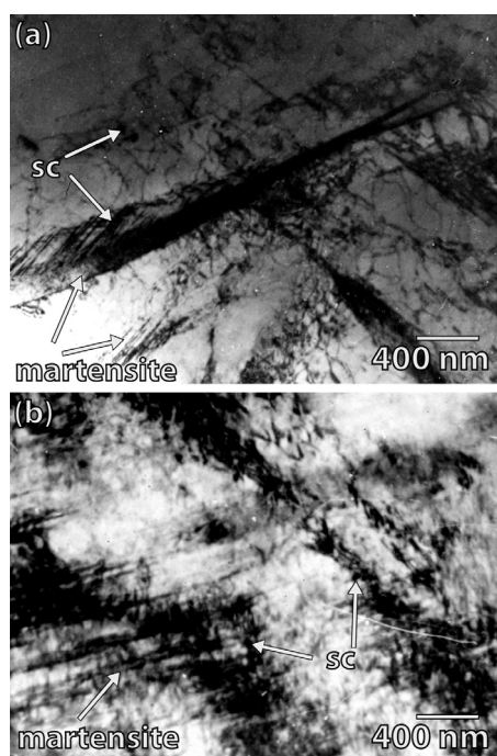
Figure 2: TEM micrographs of the: a) Fe-Cr-C-V alloy and b) Fe-Cr-C-Nb-V alloy showing secondary carbides and martensite Slika 2: TEM-posnetka: a) Fe-Cr-C-V-zlitine in b) Fe-Cr-C-Nb-V-zlitine s sekundarnimi karbidi in martenzitom
