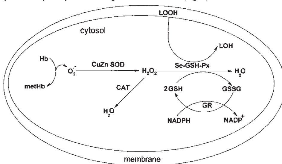
Fig. 1. A schematic representation of a part of the anti-oxidant enzyme system in erythrocytes.
