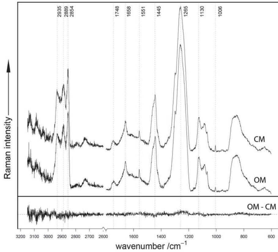
Figure 1. Mean spectrum of organic pasteurized milk (OPM) compared to mean spectra of conventional pasteurized milk (CPM) in order to investigate spectral differences by calculating the difference spectrum (OPM-CPM).
