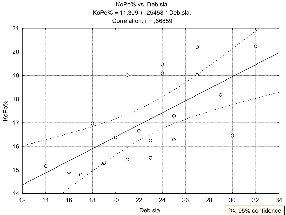
Grafikon 1. Grafički prikaz regresije udela kože sa potkožno masnim tkivom u trupu na debljinu slanine na leđjima Graph 1. Graphical presentation of the regression of share of subcutaneous fat tissue in carcass on back fat thickness
