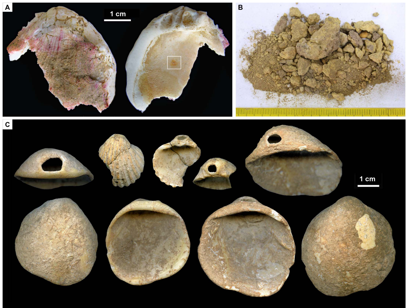
Fig. 3. Symbolic finds [after Zilhão et al. (12)]. (A) Spondylus shell with remnants (indicated by the white square) of a pigmentary compound mixing ground inclusions of hematite and pyrite in a red lepidocrocite basis. (B) Large lump of natrojarosite, a mineral whose only known archaeological use is in cosmetics. (C) Perforated Acanthocardia and Glycymeris shells (red hematite residues were found adhering to the inner side of the larger Glycymeris ).
