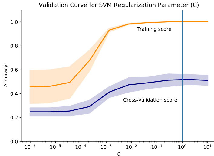
Fig. 1. Results for tuning the regularization hyperparameter ( C ) of the POS bigram SVM model. The top represents performance on the training set, while the bottom line is the cross-validation accuracy. The vertical line represents the value of C=1 .
