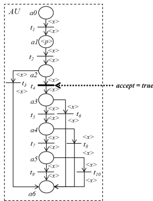
Figure 4: An possible inconsistency in a classical Workflow net.
