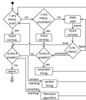
Figure 5: Possibilistic token player algorithm associated to autonomous local processes.
