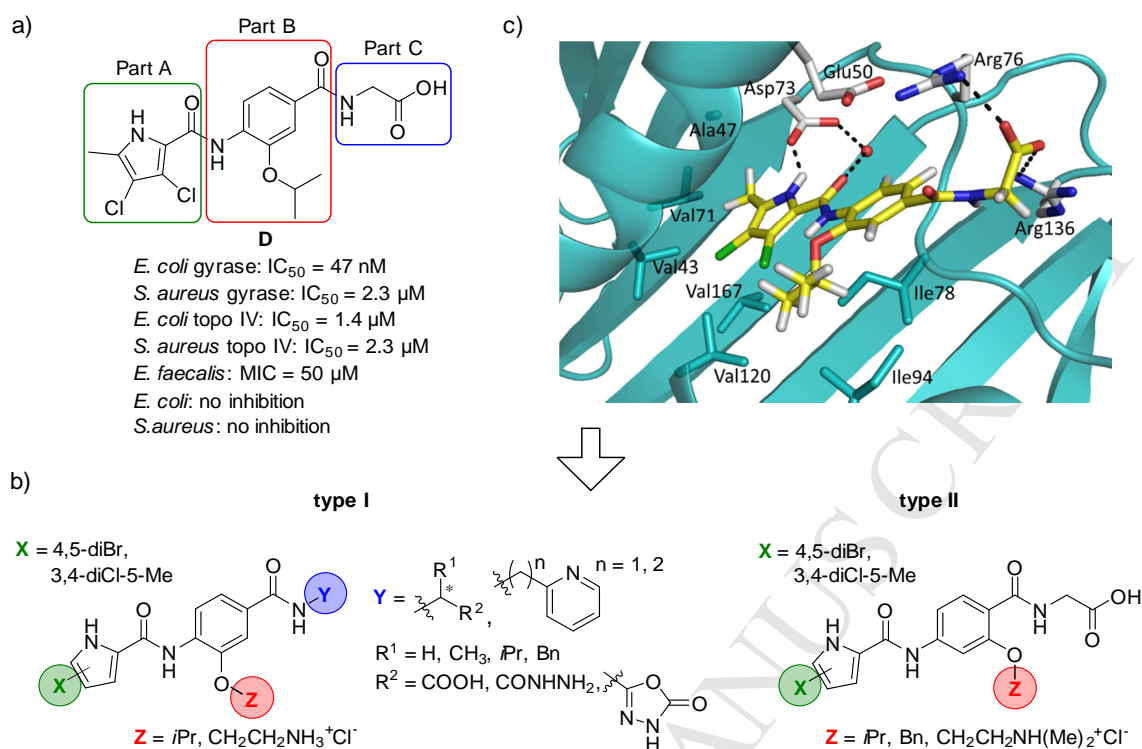
Figure 2. a) A representative N -phenylpyrrolamide D and its inhibitory activities on DNA gyrase and topoisomerase IV [16]; b) Structures of type I and type II N -phenylpyrrolamide inhibitors; c) Docking binding mode of inhibitor D coloured according to the atom chemical type (C, yellow; N, blue; O, red; Cl, green) in the ATP binding site of E. coli GyrB (in cyan, PDB code: 4DUH [22]). The water molecule is presented as a red sphere.
