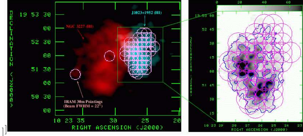
Fig. 1. Left : Location of IRAM 30m pointings (FWHM=22'') overlaid on colour image of HI emission from spiral galaxy NGC 3227 (red) and J1023+1952 (blue). Right : Location of IRAM pointings on J1023+1952, overlaid over HI emission.
