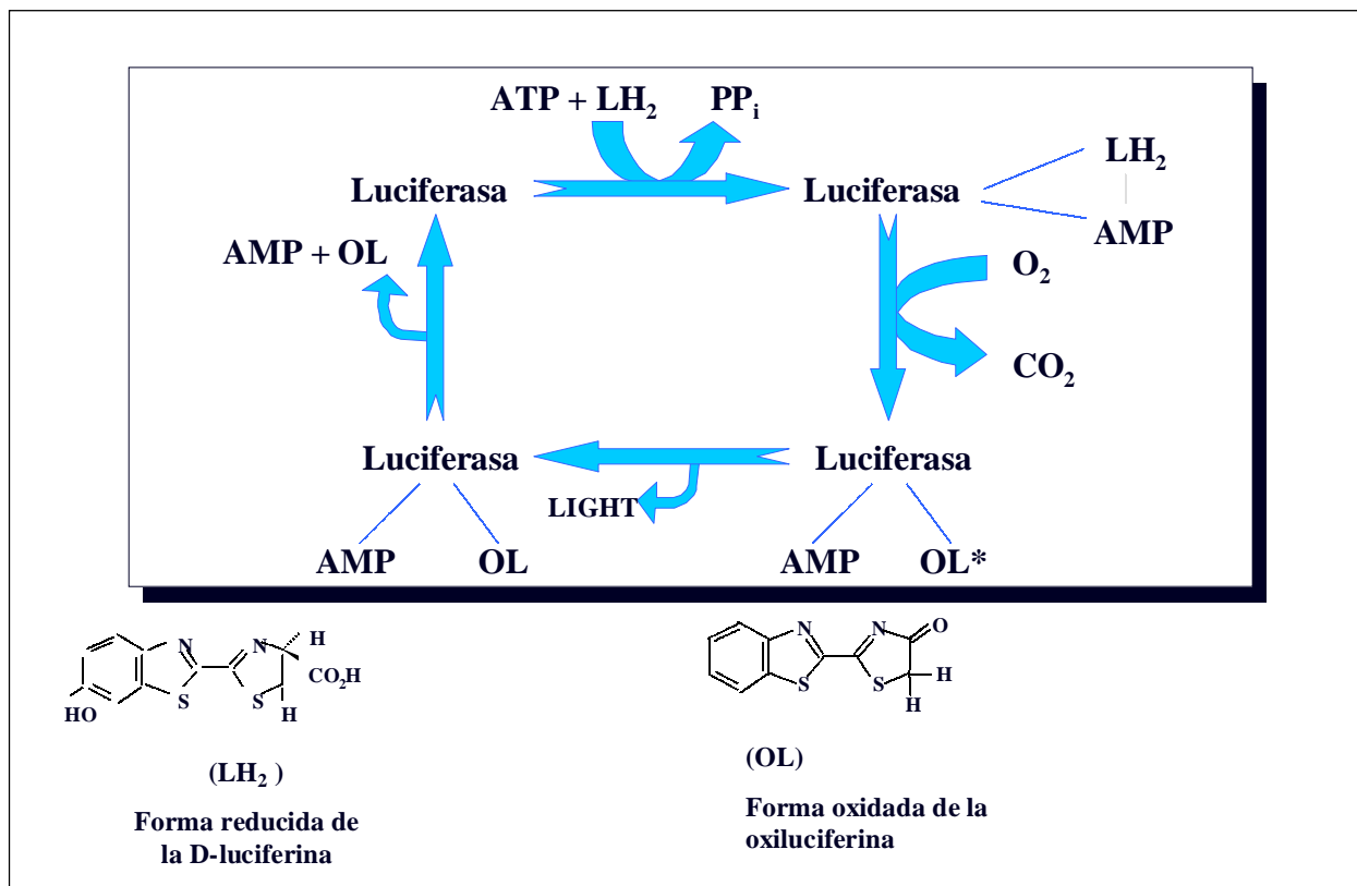
FIGURE 6.- Schematic representation of the firefly luciferase reaction. ATP, adenosine triphosphate; PP_i , pyrophosphate; AMP, adenosine monophosphate.
