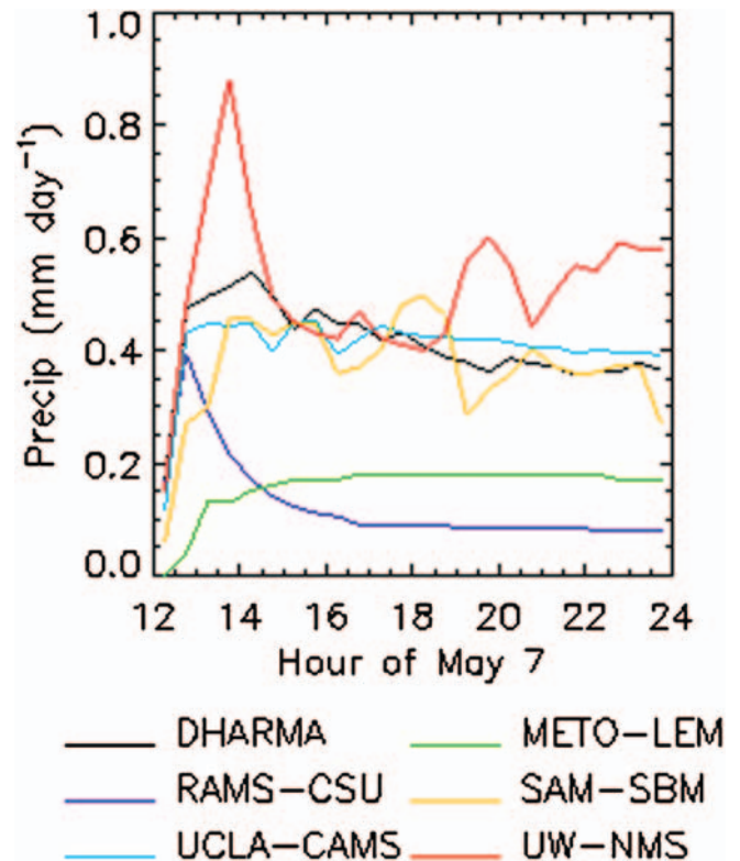
Figure 6. Timeseries of liquid-equivalent surface precipitation rates for BASE.
