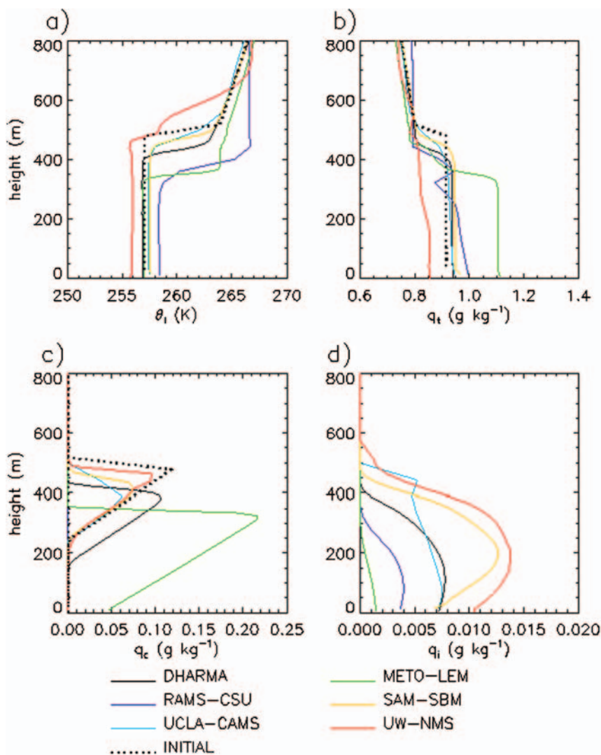
Figure 7. Horizontally-averaged vertical profiles for BASE of a) liquid water potential temperature, \theta_l , b) total water mixing ratio, q_t , c) cloud water mixing ratio, q_c , and d) ice mixing ratio, q_i , averaged between t = 11.5 to 12 h. Specified initial profiles of \theta_l , q_t , and q_c are also shown.
