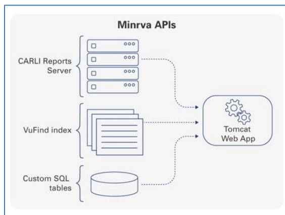
Figure 1. The data sources the Wayfinder and location-based recommendation service require.
