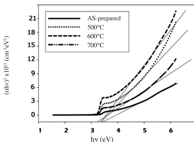
FIGURE 5. (\alpha hv)^2 vs. h\nu curves of the ZnO thin films annealed at different temperatures
