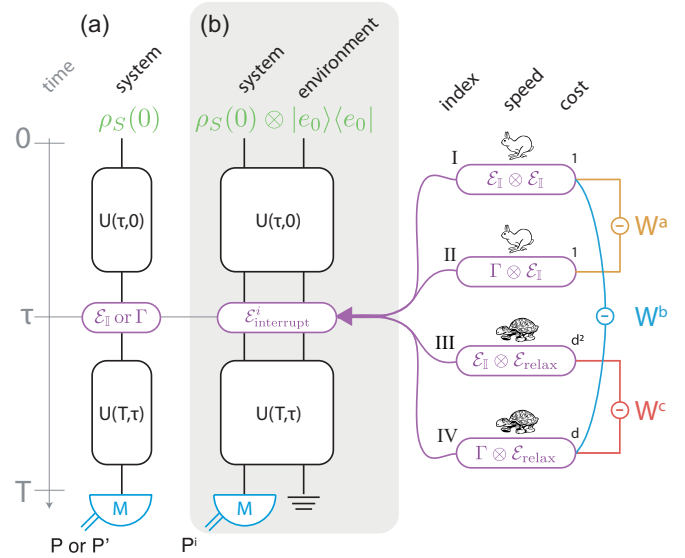
FIG. 1. Procedures for extracting coherence witnesses (time runs from top to bottom): (a) In the usual NSIT protocol the system is considered well isolated. (b) Our generalizations include an explicit environment, with each interruption experiment (fast operations i = I, II and slow operations i = III, IV ) carrying a cost in terms of the number of subexperiments required. \mathcal{E}_I is the identity channel.
