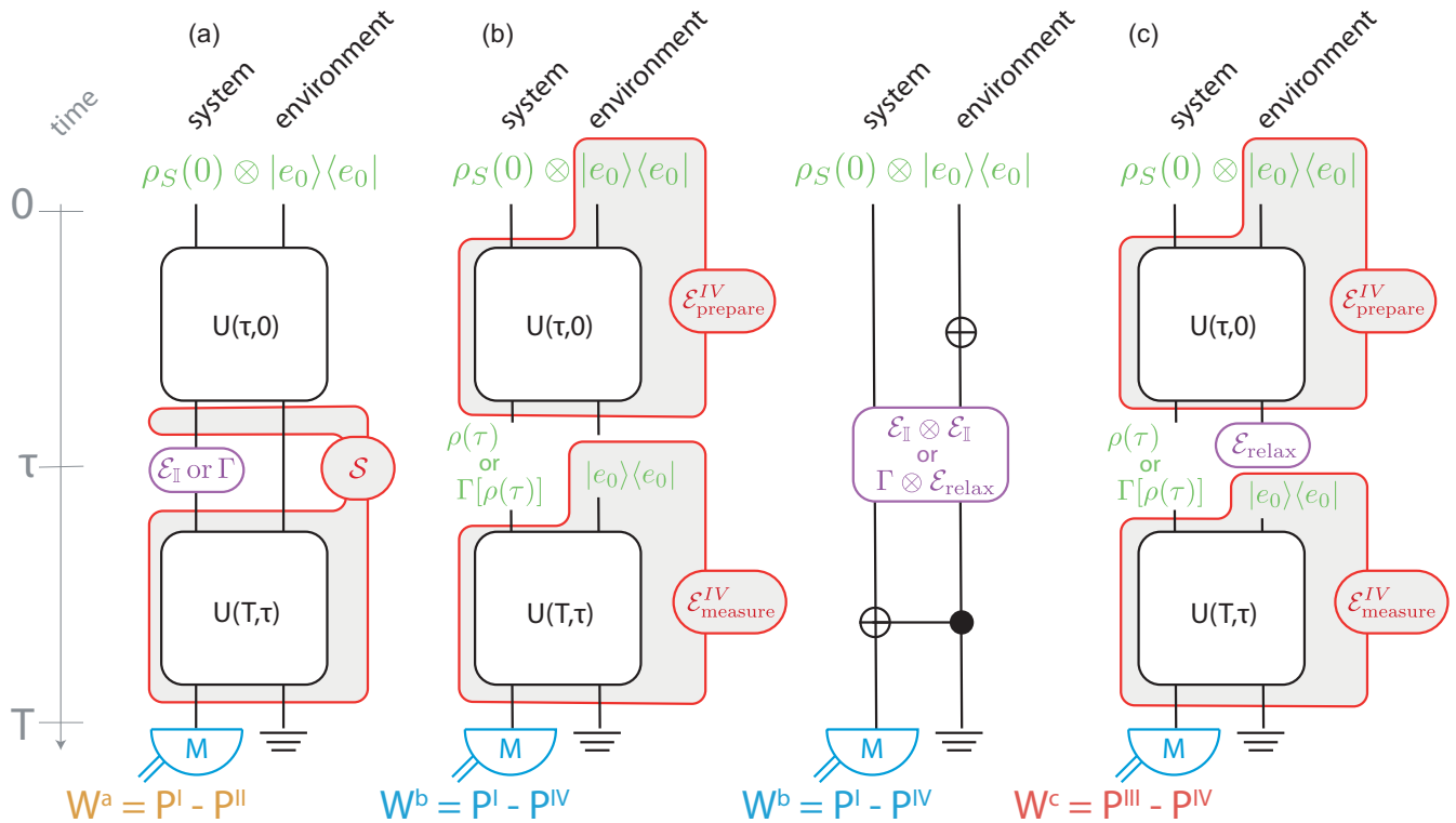
FIG. 2. (a) In the general case of a nonisolated system, it is not possible to separate preparation and measurement of the system state at \tau as is possible for an isolated system. Instead, a generalized witness compares the effect of a fixed superchannel S (which represents the combined effect of the correlated system-environment state at \tau and their joint evolution) on an input interruption channel: either the identity channel \mathcal{E}_I or the classicalization channel \Gamma [Eq. (1) or (2)] acting on the system. The associated witness W^a is sensitive to system coherence and/or quantum system-environment correlations at \tau . (b) When the Born approximation holds, the environment stays in the same state at all times and therefore need not be actively reset (left panel). \mathcal{E}_{measure}^{IV} is used to effectively alter the final measurement that is performed. Otherwise, when the Born approximation fails, classical models may explain the discrepancy between P and P' (right panel). (c) The Born approximation can be enforced by performing full quantum state tomography of the system at \tau . The associated witness W^c is sensitive only to coherence in the reduced state of the system at \tau , but requires order d^2 experiments due to the implicit full state tomography required.
