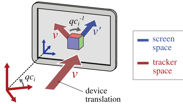
Figure 2. Directly applying the measured device translation v to the manipulated object would move it in unexpected directions, depending on the device orientation qc_i in tracker space. To get a more predictable behavior, the vector v should be rotated by the inverse rotation qc_i^{-1} , producing the correct translation v' . The same process is applied to rotations.
