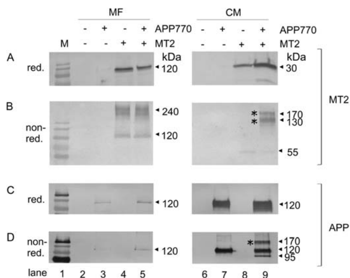
Figure 3 Stable complex formation of matriptase-2 and APP770.
