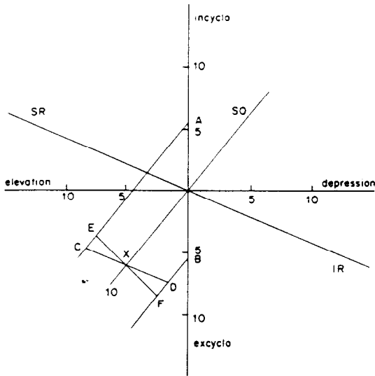
Fig. 1. Vector diagram to visualize the relation between BHT and OCR. Ordinate represents torsional eye movement. Abscissa represents vertical eye movement. Vectors of muscle action of superior rectus (SR), inferior rectus (IR), superior oblique (SO) and inferior oblique (IO) are drawn. Points A and B represent the positions the eye assumes in OCR, 5\frac{1}{2} deg incyclo and 5\frac{1}{2} deg excylo, on average. If the SO is paralysed, the eye will move in a direction opposite to the SO vector (point X). The positions the eye will assume on head-tilt will shift in a similar direction (points E and F). In the case drawn, a VD of 5 deg and an excyclotropia of 6 deg is assumed. What is the path the eye will take in BHT? CD is parallel to the SR and IR vectors. As the IO is still working, EF would then seem a reasonable guess, with a change in VD of 5 deg and a change in excyclotropia of 6 deg. Note that differences in vertical and torsional stiffness of the eye have not been taken into account (Simonsz et al. , 1984).
