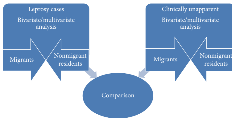
FIGURE 2: Study design.
