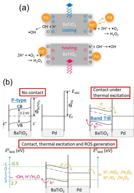
Fig. 6 (a) Schematic of reactive oxygen species (ROS) generation driven by the pyro-electro-chemical effect assisted by palladium nanoparticles. 32 (b) Energy level diagrams and reactive oxygen species (ROS)-generating charge transfer due to thermal excitation of pyroelectric barium titanate. Redox potentials between palladium nanoparticles, barium titanate, and neutral aqueous surrounding relative to standard hydrogen electrode are compared for selected species. Adapted with permission from Ref. 32. Copyright (2015) American Chemical Society.
