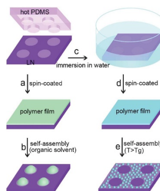
Fig. 11 Schematic showing the procedure of electrostatic charge patterning using hot micro-contact printing on LiNbO 3 (LN) substrate followed by self-assembly of thin polymer film. Reproduced from Ref. 47 with permission from The Royal Society of Chemistry.
