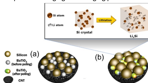
Fig. 20 Schematic of microstructural changes in the Si/carbon nanotube (CNT)/BaTiO 3 nanocomposite anode during lithiation. (a) Si and BaTiO 3 particles are dispersed and attached to the CNT. (b) Lithiation of Si results in a large increase in volume, pressurising BaTiO 3 nanoparticles to create a piezoelectric potential. Adapted with permission from Ref. 84. Copyright (2016) American Chemical Society.
