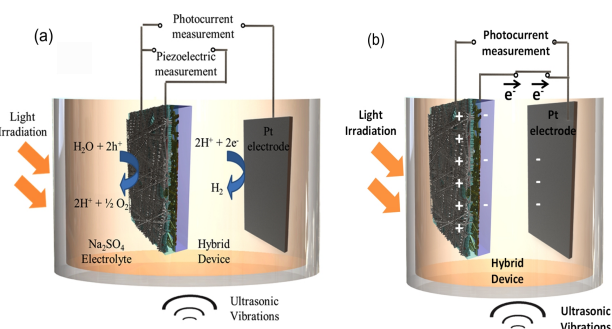
Fig. 14 Operation of the hybrid device (a) Individual piezoelectric and photocurrent measurement (b) Charge transfer during deformation of the piezoelectric and photo-catalytic electrode under ultrasonic vibration and light irradiation. Reprinted with permission from Ref. 55. Copyright (2015) American Chemical Society.
