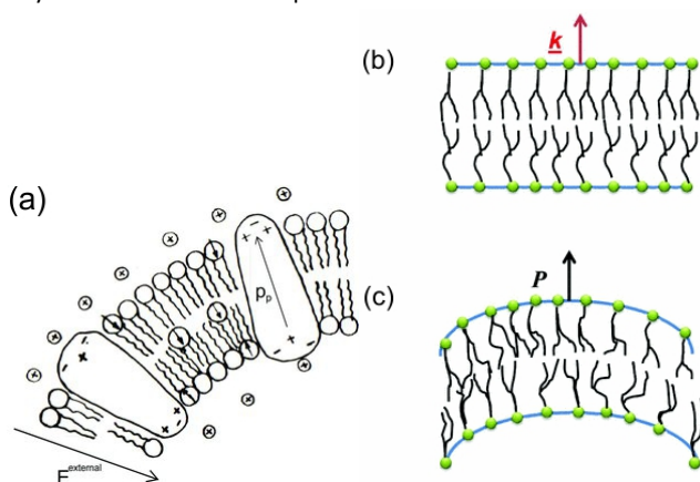
Fig. 28 Flexo-electricity in biological membranes. (a) Schematic of bilayer lipid membrane under external electrical field, and globular proteins with an intrinsic polarisation. Ref. 152- Copyright 1975, with permission of Springer. (b) Under planar conditions there is no polarisation and (c) Under bending the lower surface is in compression and the upper one in dilation, and an electric polarisation is generated. Reprinted figure with permission from Ref. 153 . Copyright (2013) by the American Physical Society.
