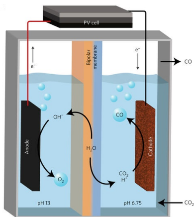
Fig. 38 Schematic of solar-driven CO 2 reduction device. Anode: reaction: 2\text{OH}^- \rightarrow \text{H}_2\text{O} + \frac{1}{2}\text{O}_2 + 2\text{e}^- ; cathode reaction: \text{CO}_2 + 2\text{H}^+ + 2\text{e}^- \rightarrow \text{CO} + \text{H}_2\text{O} . Reprinted by permission from Macmillan Publishers Ltd: Ref. 209 (Copyright 2017).
