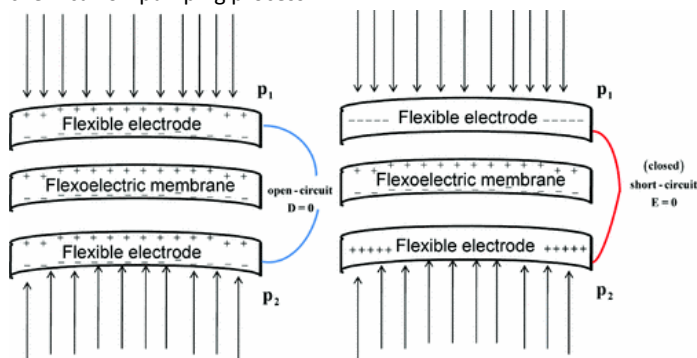
Fig. 32 Open ( D=0 ) and closed circuit ( E=0 ) states for a flexoelectric membrane under bending. P shows pressure. Reprinted figure with permission from Ref. 153. Copyright (2013) by the American Physical Society.
