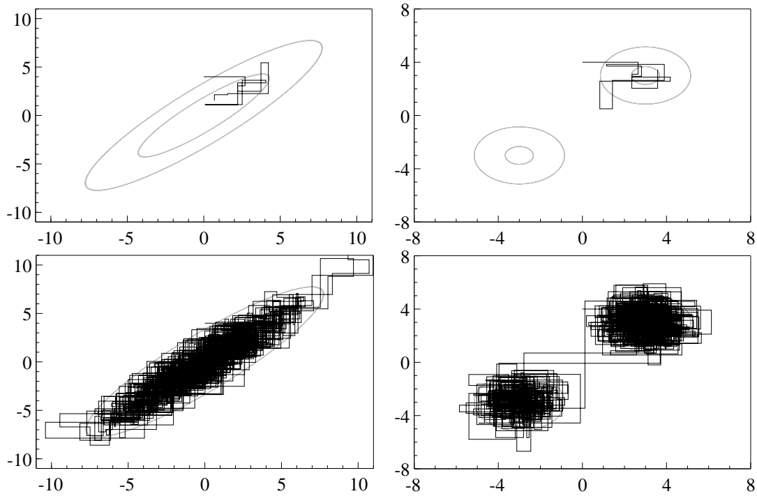
Figure 5.4: Illustration of the Gibbs sampler for a correlated target density (left) and a bimodal target density (right). The generated sample paths are shown for 10 iterations (above) and 1000 iterations (below).
