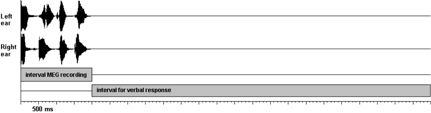
Fig. 1. Schematic representation of dichotic stimuli and task over time
