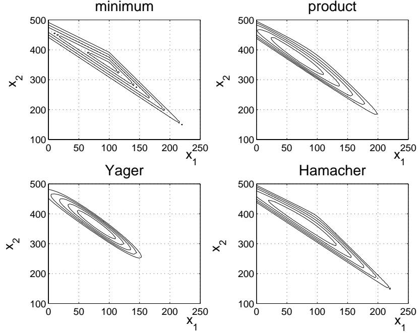
Figure 3: Regions within which the optimal solution is sought for different fuzzy aggregation operators.
