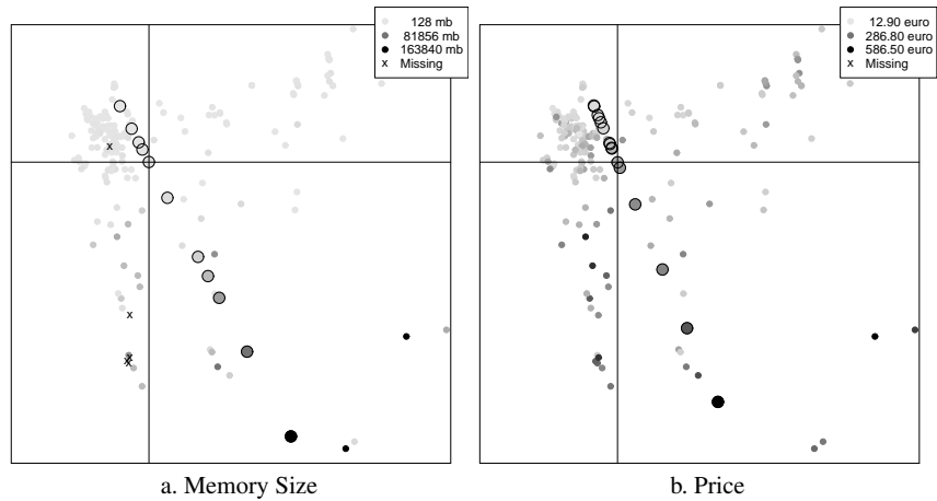
Fig. 10 Biplots based on NL-PCA labeled by Memory Size and Price. Large circles are category points and small dots represent object points.
