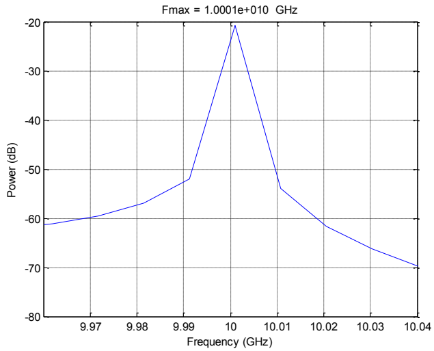
Figure 4-7: Electrical spectrum
