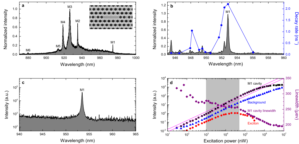
Fig. 1. Few-QD nanolasing. (a) Spectrum of an L3 cavity with embedded QDs at high-power (1 mW) above-band excitation showing the characteristic cavity modes denoted M1-M6. The inset shows a scanning-electron micrograph of the sample. (b) Spectrum (black curve; left axis) around the M1-cavity obtained with M6-resonant excitation at 100 nW showing the M1 cavity mode and a number of excitonic peaks whose decay rates (blue circles; right axis) have been measured using time-resolved spectroscopy. (c) Spectrum around M1 obtained with M6-resonant excitation at 100 \mu W showing the M1-cavity peak on a pronounced background. (d) Integrated intensity as a function of excitation power for the M1-cavity mode (black squares), an exciton peak (red circles), and the background (blue triangles). The smooth s-shaped transition between linear regions (magenta lines) of the cavity power dependence is a characteristic signature of high- \beta lasing. Evidently, the exciton saturates around threshold (gray region) and cannot provide the gain for the laser, which is provided by the background. The linewidth (purple diamonds; right axis) shows a small narrowing consistent with high- \beta lasing.
