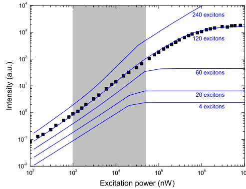
Fig. 2. Comparison of the experimental (black squares) and theoretical (blue lines) input-output curves. Clearly, the model cannot fit the data for small numbers of emitters although only four excitons were found to be coupled to the cavity at low excitation power. By varying the number of emitters in the model as indicated in the plot we find that 120 emitters must be included to fit the experiment. The theoretical curves have been vertically offset for clarity.
