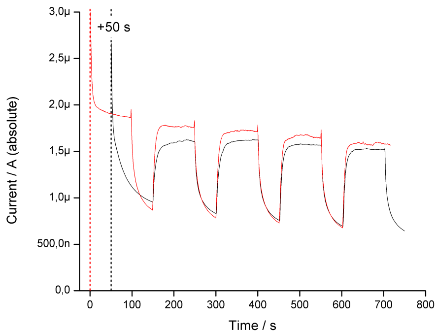
Figure 23.5: Amperometric measurements on a series of spinning and stopping the disc initially rotating (red line) and static (black line) at 30 RPM. Courtesy of Sune Zoëga Andreasen.
