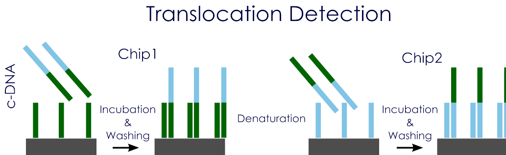
Figure 17.8: Schematic of a double hybridisation assay on silicon nanowires. For the experiment two chips were used with Chip1 covered with 9.3 probes and Chip2 with 9.9 probes. After incubation with a DNA fragment complementary to the probes on Chip1, the captured fragment was released and incubated with the probes on Chip2.
