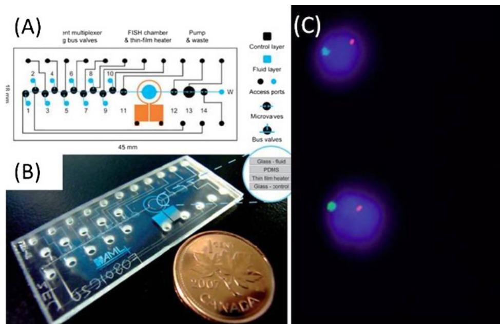
Fig. 4 (A) The mask layouts and dimensions of an integrated FISH microchip. The microchip includes a reagent multiplexer, a cell chamber with an integrated thin-film heater, and a peristaltic pump. (B) Image of a complete integrated FISH chip. (C) Interphase FISH results of a male sample showing signals from one X and one Y chromosomes (used with permission from (Sieben et al. 2008))
