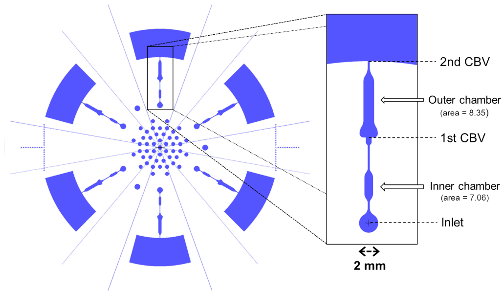
Figure 22.2: Design of microfluidics on a disc with a zoom in to one of the channels with all channel features marked. Courtesy of Sune Zoëga Andreasen.
