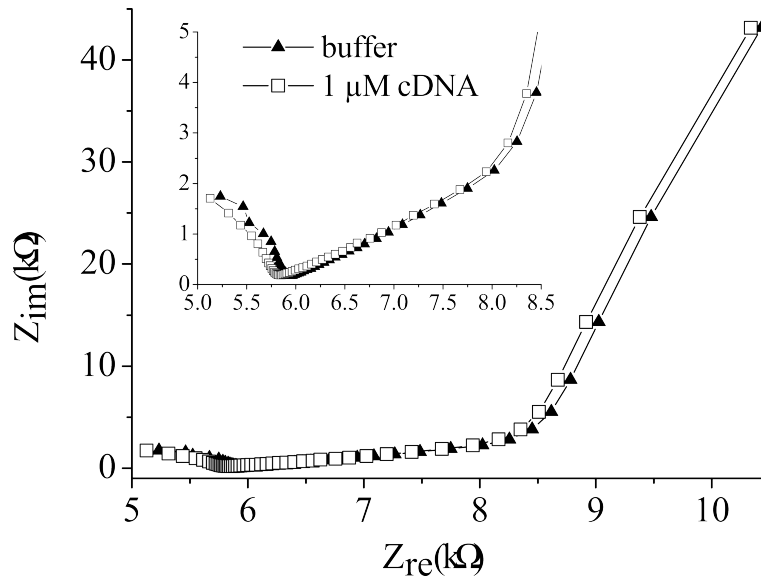
Figure 19.3: Nyquist plot of two impedance spectra before (triangles) and after (squares) injection of complementary DNA. The inset shows the high frequency part of the spectra in detail.
