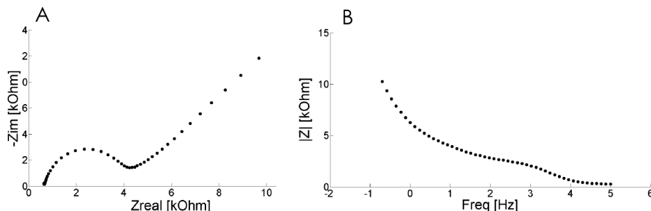
Figure 18.1: Typical EIS plots - a Nyquist plot on the left (A) and a Bode Modulus plot on the right (B).
