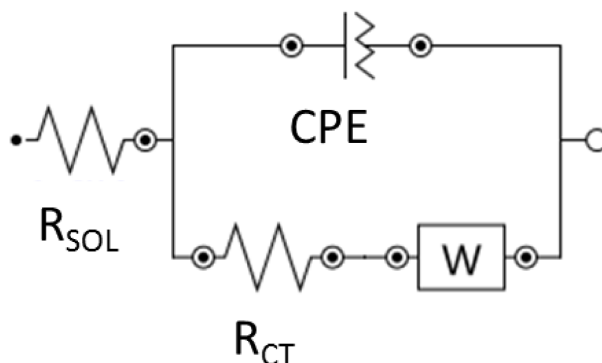
Figure 18.2: Randles circuit with a constant phase element.
