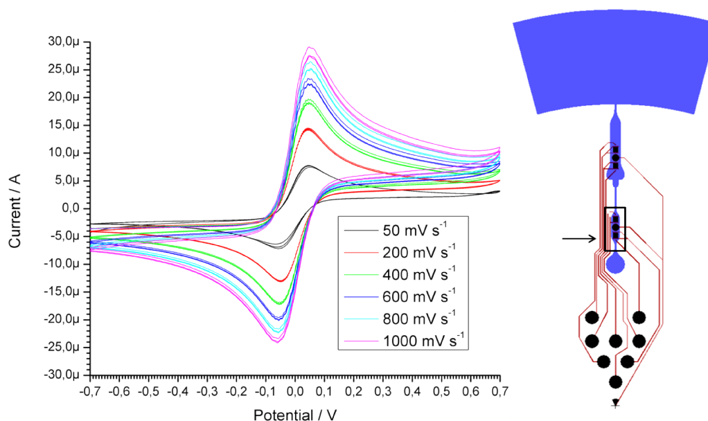
Figure 23.1: Overlay of series of CVs at different scan rates (left) with a scheme of the electrodes position (right). Courtesy of Sune Zoëga Andreasen.
