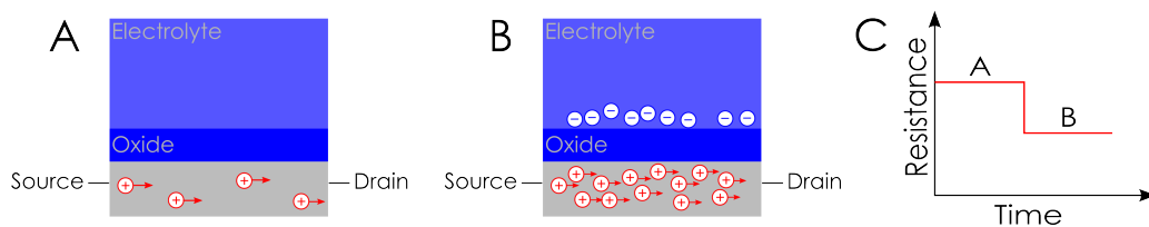
Figure 17.1: Principle of detection with p-type SiNW. The holes as charge carriers appear to be running from source to drain in the p-type nanowire (A). When negatively charged particles are introduced in the electrolyte more holes are attracted from the bulk (B). The nanowire resistance change is shown in C with an initial stable value that decrease when the negatively charged particles are added.
