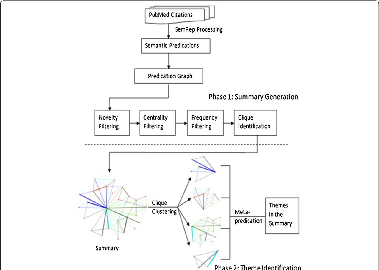
Figure 3 Work flow of the summarization processing. The system includes two phases in processing. In the first phase, semantic predications extracted from MEDLINE citations with SemRep are represented in a graph. Then four processing steps (novelty filtering to eliminate uninformative predications, node centrality filtering, frequency filtering, and clique identification) successively condense the predication graph into a graphic summary. In phase two, clique clustering, an application of the UCINET, is used to partition the summary into several clusters representing summary themes. The theme of the clusters is labeled with a metapredication.
