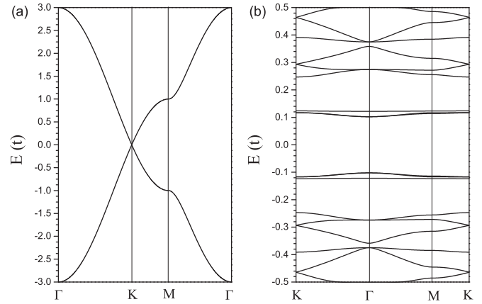
FIG. 2. Band structure of SLG (a) and of a \{10,6\} GAL (b).
