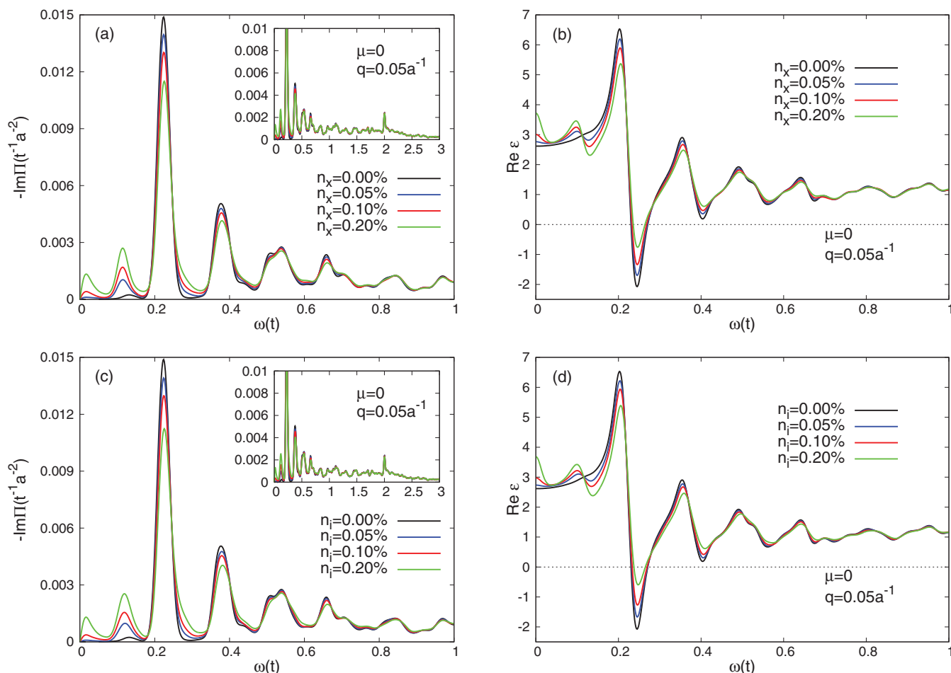
FIG. 8. (Color online) Same as shown in Fig. 4 but in the presence of resonant impurities. Panels (a) and (b) correspond to \text{Im}\Pi(q, \omega) and \text{Re}\epsilon(q, \omega) , respectively, for a {10,6} GAL with a random distribution of vacancies. The different colors correspond to different amounts of missing dangling bonds, as denoted in the inset of the figures. Panels (c) and (d) corresponds to a GAL with hydrogen adatoms. Different colors correspond to different percentage of adatoms in the sample. The insets in panels (a) and (c) show the polarization in a broader range of energies.
