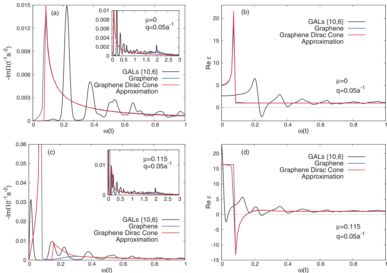
FIG. 4. (Color online) Comparison between SLG and GALs. Polarization function [(a) and (c)] and dielectric function [(b) and (d)] for a {10,6} GAL. Black lines correspond to GAL, whereas the blue lines correspond to SLG within the \pi -band tight-binding model, and the red lines correspond to SLG using the Dirac cone approximation. Panels (a) and (b) are for undoped samples ( \mu = 0 ), and panels (c) and (d) are for doped samples with \mu = 0.115t . The insets in (a) and (c) give the spectra in a broader range of energies.
