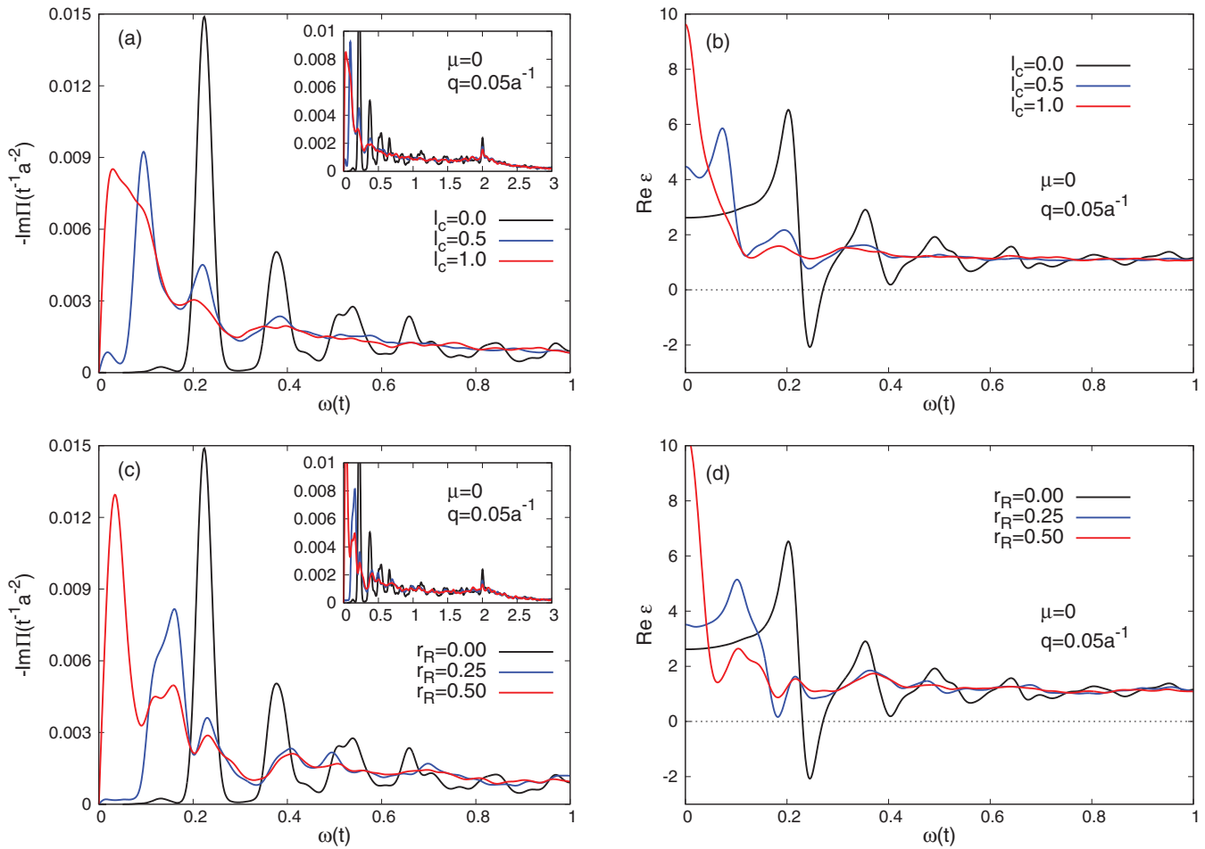
FIG. 7. (Color online) Same as shown in Fig. 4 but in the presence of geometrical disorder. Panels (a) and (b) corresponds to \text{Im}\Pi(q, \omega) and \text{Re}\varepsilon(q, \omega) , respectively, for a GAL in which the center of the holes is shifted randomly with respect to the original position in the perfect periodic array, within the range (x \pm l_c, y \pm l_c) . The different colors correspond to different values of l_c (in units of a ), as denoted in the inset of the figures. Panels (c) and (d) corresponds to a GAL where the radius of the holes is randomly shrunk or enlarged within the range [R - r_R, R + r_R] . Different colors correspond to different values of r_R (in units of a ). The insets in panels (a) and (c) show the polarization in a broader range of energies.
