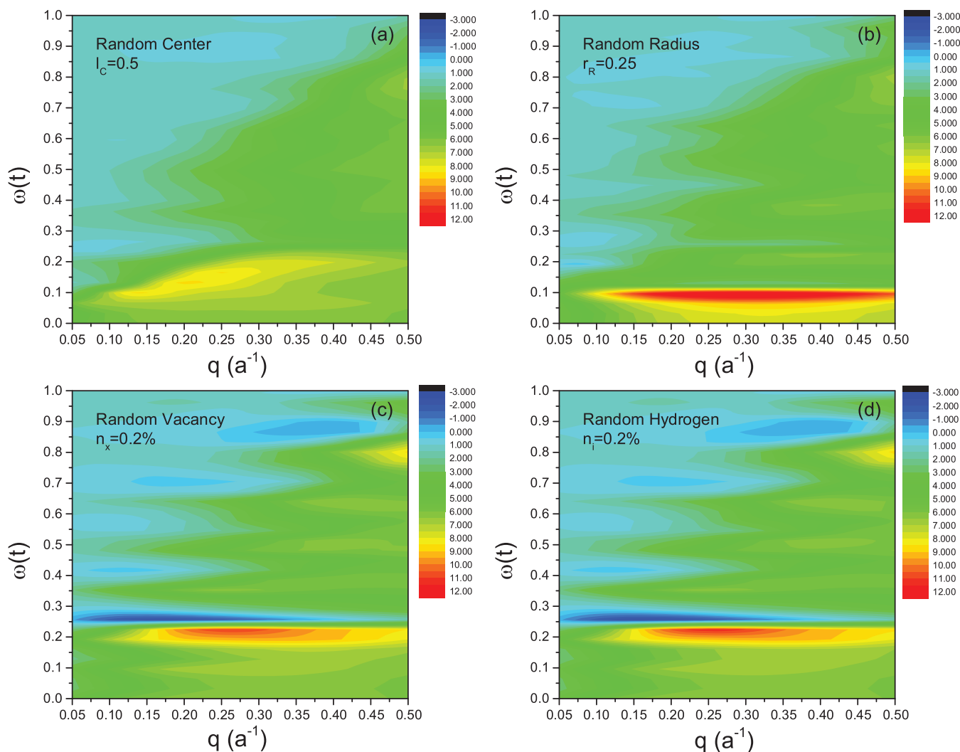
FIG. 6. (Color online) Density plot of \text{Re}\varepsilon(q, \omega) for four different types of disorder. (a) Random center; (b) random radius; (c) random vacancies; (d) random hydrogen adsorbants. The parameters characterizing the disorder are indicated in the figures.
