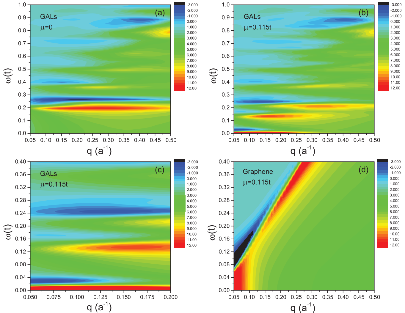
FIG. 5. (Color online) Density plots of \text{Re}\varepsilon(q, \omega) . (a) Undoped ( \mu = 0 ) GAL with \{10,6\} periodicity. (b) Doped GAL with \mu = 0.115t . (c) Same as (b) for a reduced region of the spectrum corresponding to small wave vectors and frequencies. (d) Doped SLG with \mu = 0.115t . Notice the different scales of frequencies and momenta in each plot. The plots start at q = 0.05/a . 43
