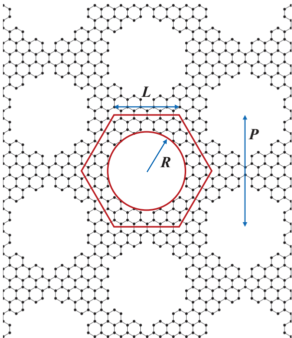
FIG. 1. (Color online) Sketch of a GAL, with the set of geometrical parameters that are used to define it as explained in the text.
