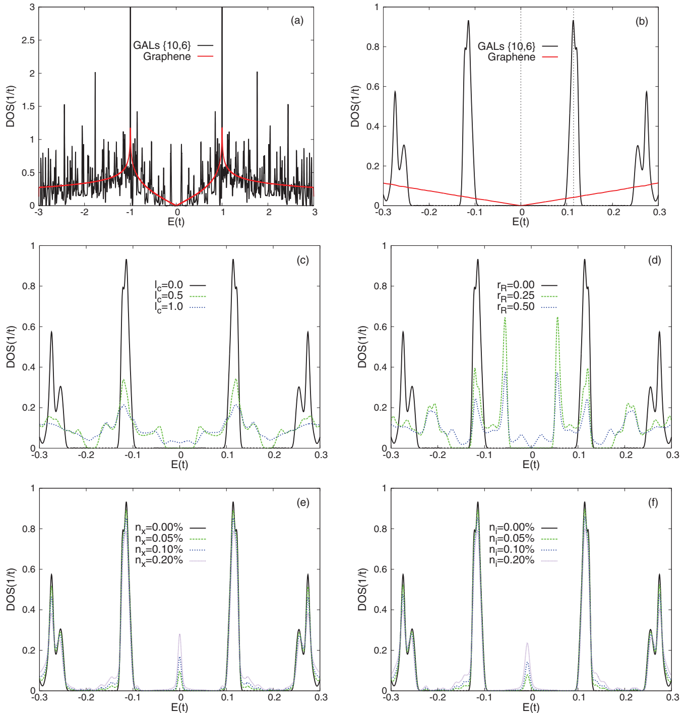
FIG. 3. (Color online) (a) DOS of a {10,6} GAL (black lines) and of SLG (red lines). (b) Same as (a) but zoomed in at low energies. (c) Random shift of the center of the antidots within the range (x \pm l_c, y \pm l_c) . (d) Random variation of the antidot radius within the range [R - r_R, R + r_R] . (e) Random vacancies for four concentrations. (f) Random hydrogen adsorbants for four coverages. The dotted vertical lines in panel (b) correspond to the two different Fermi energies considered in this work: undoped GAL with \mu = 0 and doped GAL with \mu = 0.115t .
