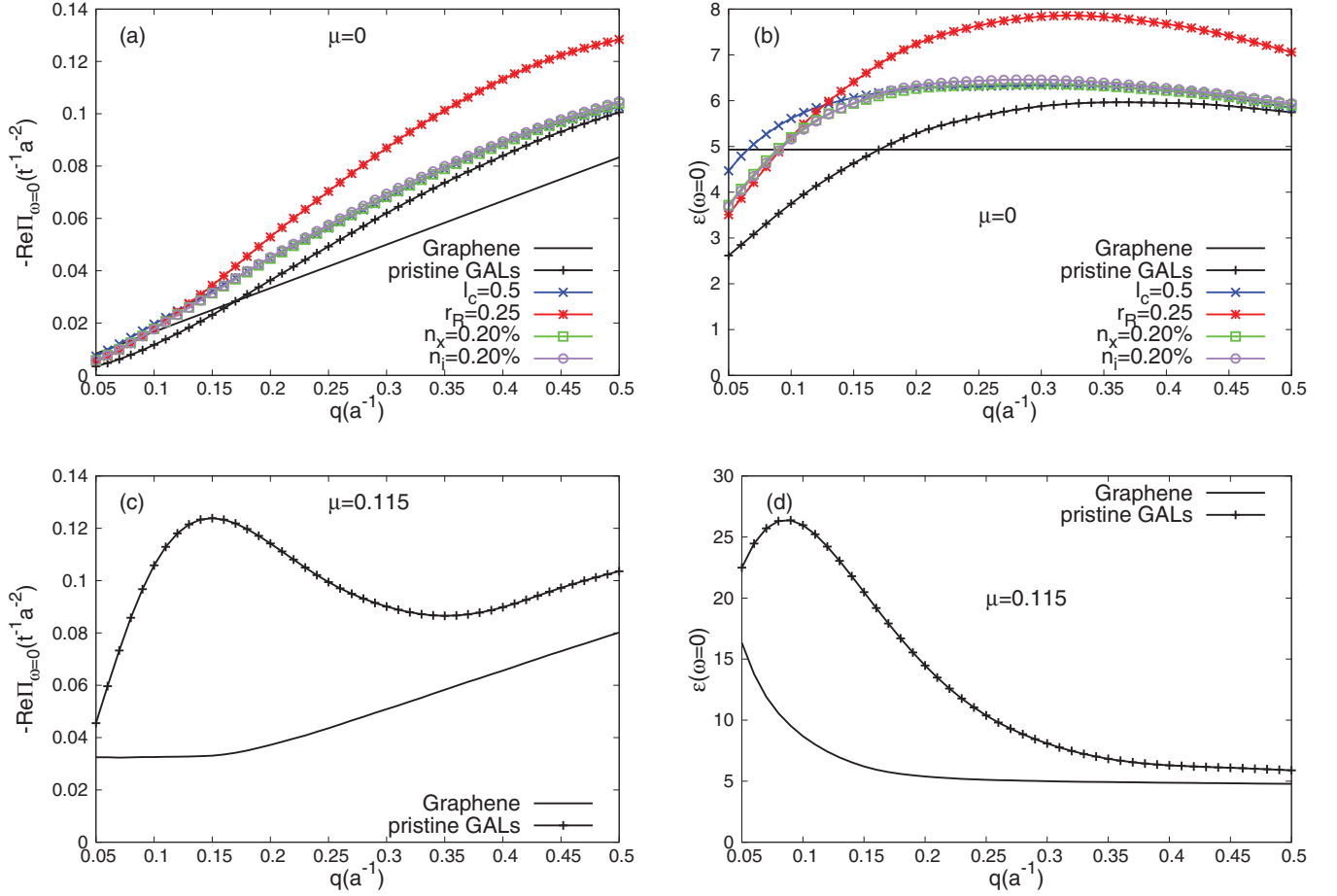
FIG. 9. (Color online) Static polarization \Pi(q, \omega = 0) and static dielectric function \varepsilon(q, \omega = 0) of GALs. Plots (a) and (b) are for undoped samples, \mu = 0 , whereas plots (c) and (d) correspond to a finite doping \mu = 0.115t . Different kinds of disorder are considered in panels (a) and (b), as described in the inset. For comparison, we include the corresponding polarization and dielectric function for SLG, as given by the full black lines in each plot.
