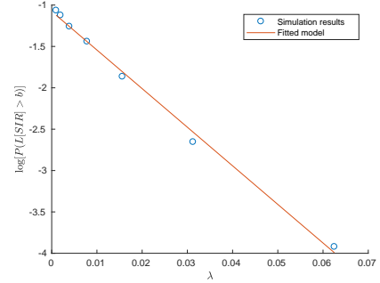
Fig. 5. Simulation estimate of \log \mathbb{P}(L_\lambda[\text{SIR}] > b) with \tau = -50 dB and \epsilon = 0.05 , fitted to a linear model \hat{y}_1 = p_1\lambda + p_2 , where p_1 = -46.65 and p_2 = -1.077 . The value of -p_1 is an estimate for the rate function.
