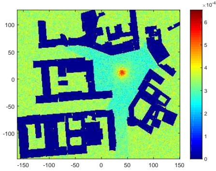
Fig. 7. Heat map of bad user configurations with simulation parameters \epsilon = 0.3 and \lambda = 2^{-12} (or \lambda \approx 2.44 \times 10^{-4} ), and \tau = -50 (or \tau_\lambda = -13.88 ) dB. The average user density is estimated for the atypical event of a large fraction of disconnected users. The regions of higher values show where users tend to be located during bad configurations. Naturally, these include regions far or hidden from the target base station. But there is also a region around the base station, due to the so-called near-far effect, where too many users have decreased the SIR values of the remaining network users.
