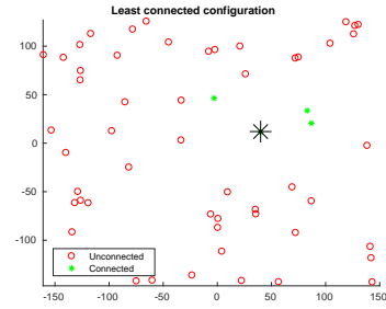
Fig. 8. The least connected configuration (7.02% connected) of a Poisson point process with density \lambda = 0.001 and \tau = -60 (or \tau_\lambda = -30 ) dB.
