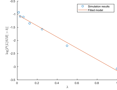
Fig. 3. Simulation estimate of \log \mathbb{P}(L_\lambda[\text{SIR}] > b) with \tau = -50 dB and \epsilon = 0.01 , fitted to a linear model \hat{y}_1 = p_1\lambda + p_2 , where p_1 = -2.138 and p_2 = -1.014 . The value of -p_1 is an estimate for the rate function.
