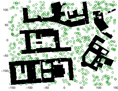
Fig. 2. A Poisson point process with density \lambda = 0.01 representing users scattered around Hausvogteiplatz in Berlin, away from buildings.
