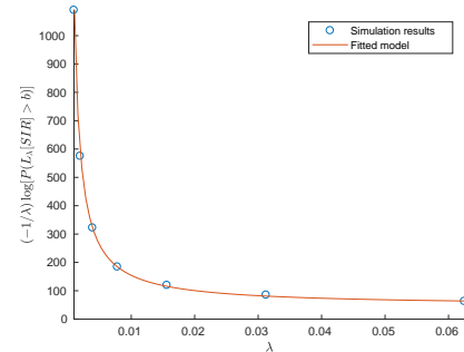
Fig. 6. Simulation estimate of -\log \mathbb{P}(L_\lambda[\text{SIR}] > b)/\lambda with \tau = -50 dB and \epsilon = 0.05 , fitted to a model \hat{y}_2 = -p_1 - p_2/\lambda , p_1 = -46.65 and p_2 = -1.077 .
