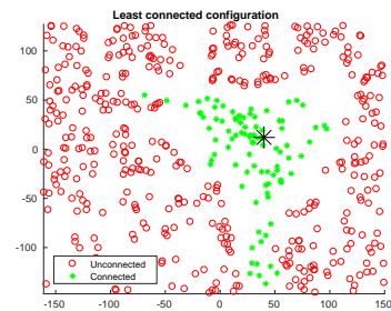
Fig. 10. The least connected configuration (17.99% connected) of a Poisson point process with density \lambda = 0.01 and \tau = -60 (or \tau_\lambda = -40 ) dB.
