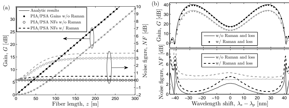
Fig. 2. (a) PIA (gray) and PSA (black) gains and NFs versus fiber length with and without the Raman effect and loss (the gain with Raman and loss are not shown; line styles apply to both PIA and PSA curves), (b) Gain and NF spectra at the amplifier output ( z = 300 m), which show the effect of SRS and LIN on the NF. Parameters: P_{p,0} = 1.4 W, P_{s,0} = 10^{-7} W, \lambda_p = 1560.7 nm, \lambda_0 = 1559 nm, \gamma = 11 (W km) ^{-1} , \partial D/\partial \lambda = 0.03 ps/(nm ^2 km), \alpha = 0.4 dB/km, T = 300 K, and \Delta z = 1 m.
